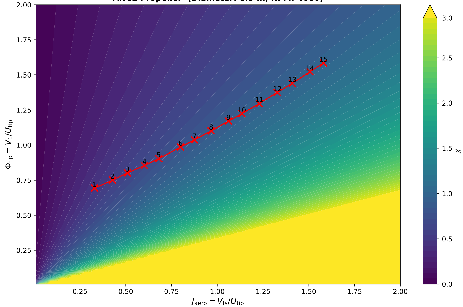
ANCE Propeller (Diameter: 8.5 in, RPM: 4000)
