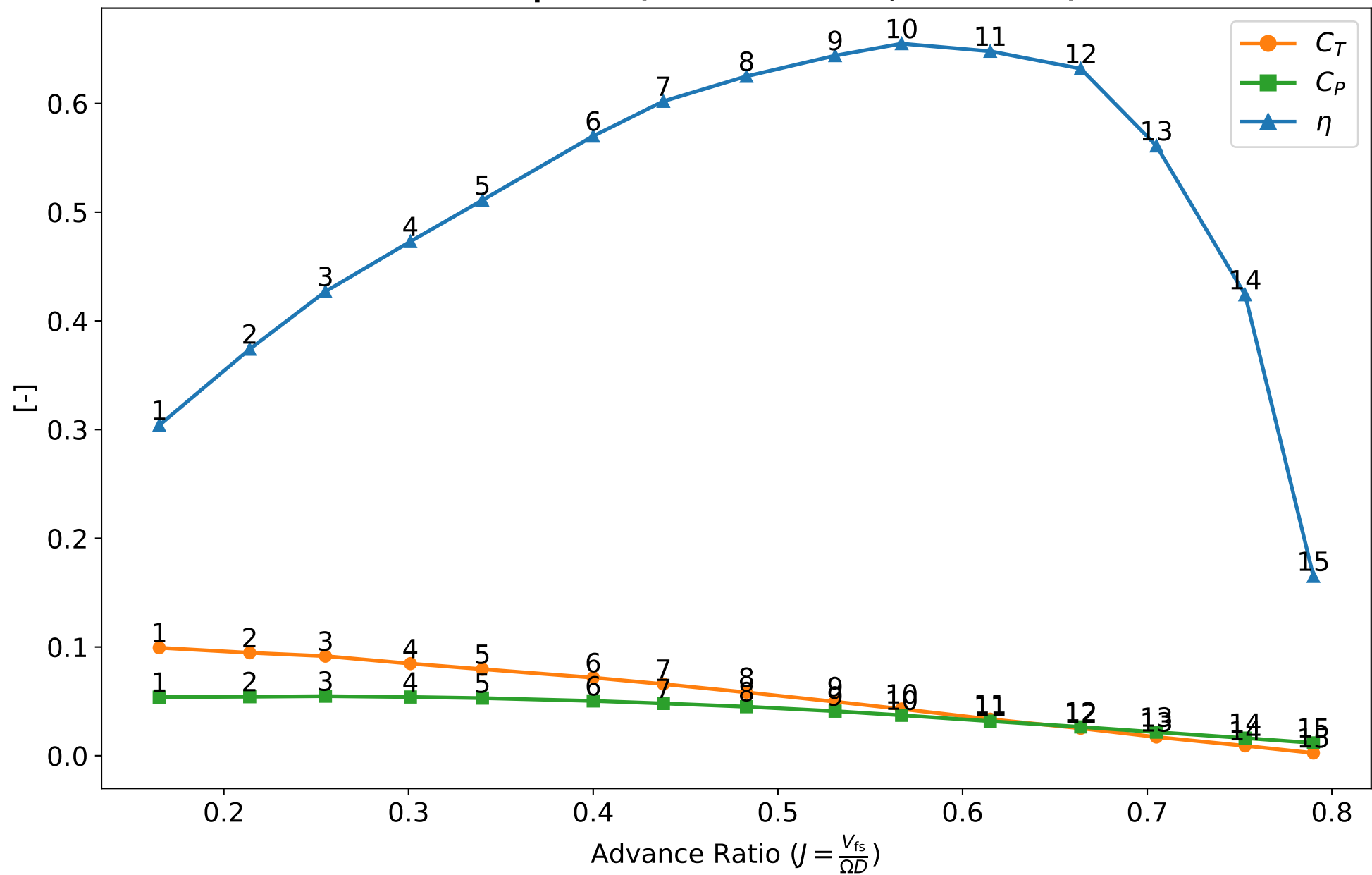
ANCE Propeller (Diameter: 8.5 in, RPM: 4000)
