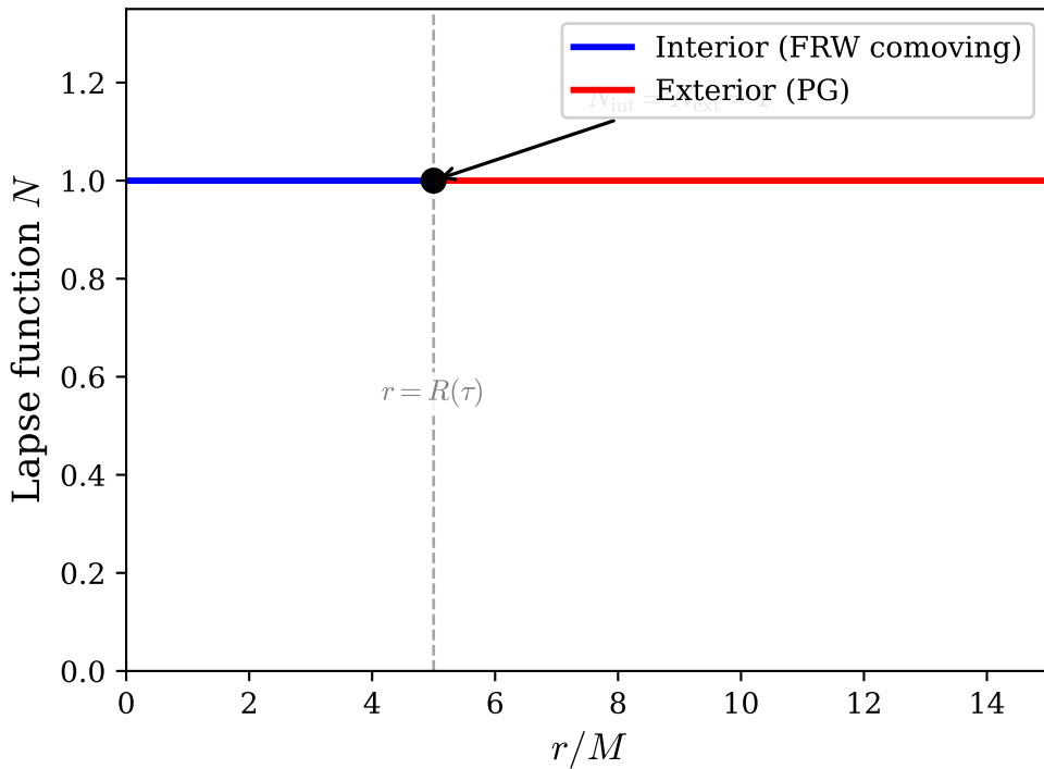
(a) N=1 gauge (PG exterior)
