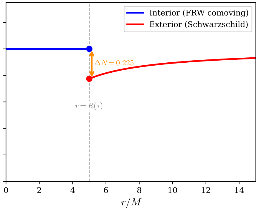
(b) Diagonal gauge (Schwarzschild exterior)
