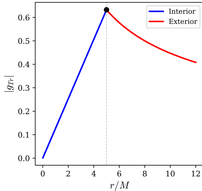
(b) |g_{Tr}| = |v|
