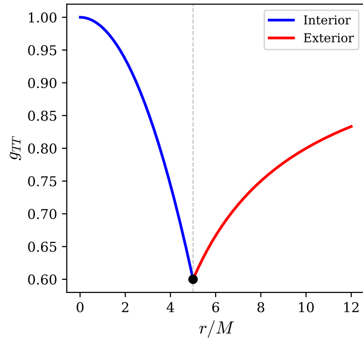
(a) g_{TT} = 1 - v^2
