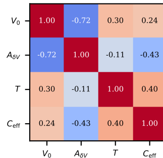
Pooled
