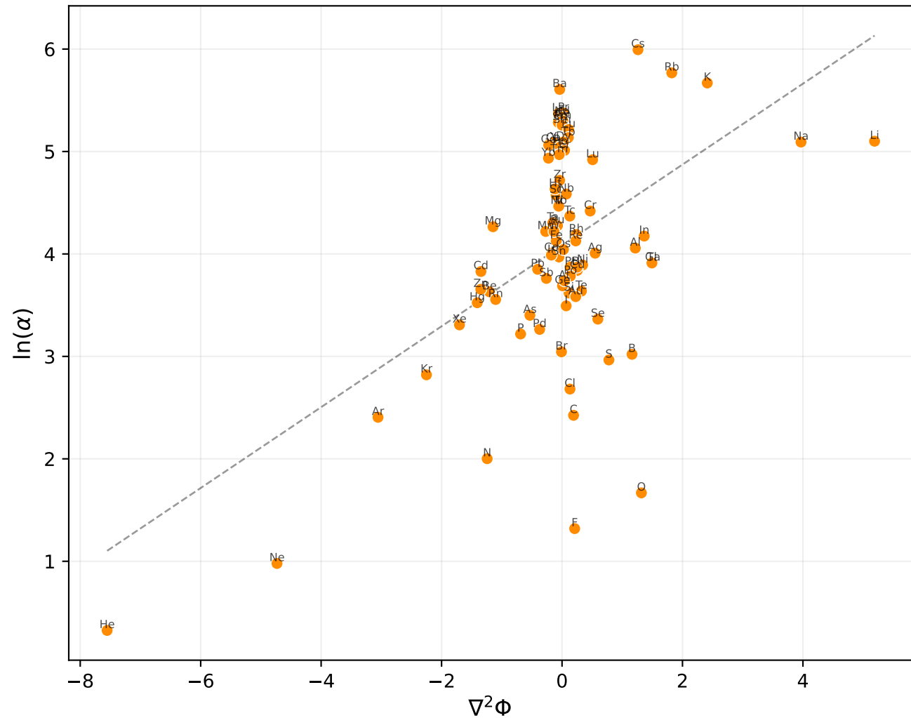
(b) Curvature vs \ln(\text{polarizability}) Pearson r = 0.533 , p = 1.5\text{e-}07 , N = 85
