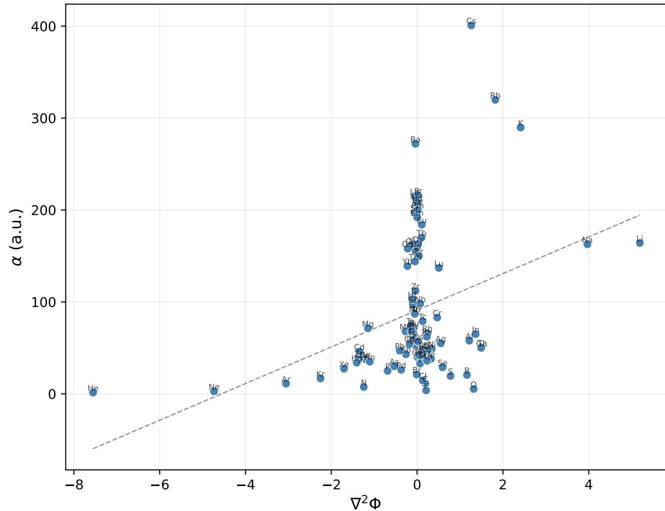
(a) Curvature vs polarizability Pearson r = 0.363 , p = 6.3\text{e-}04 , N = 85
