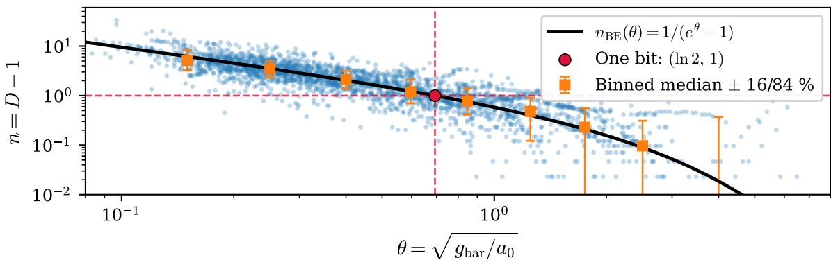
(c) Occupation number across the full \theta range
