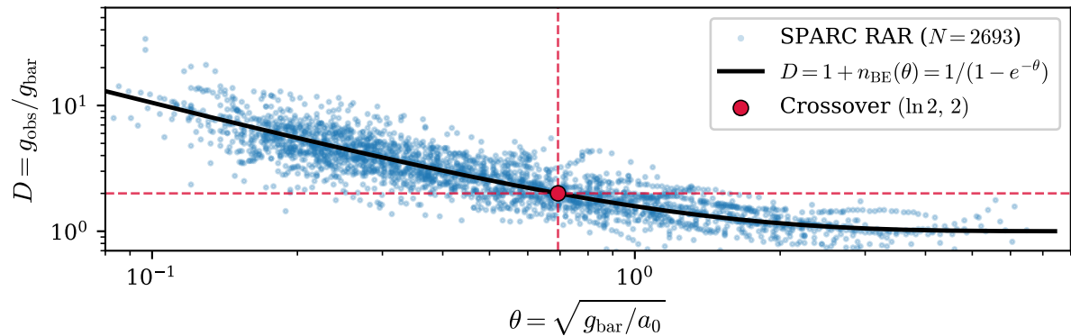
(a) Mass discrepancy across the RAR
