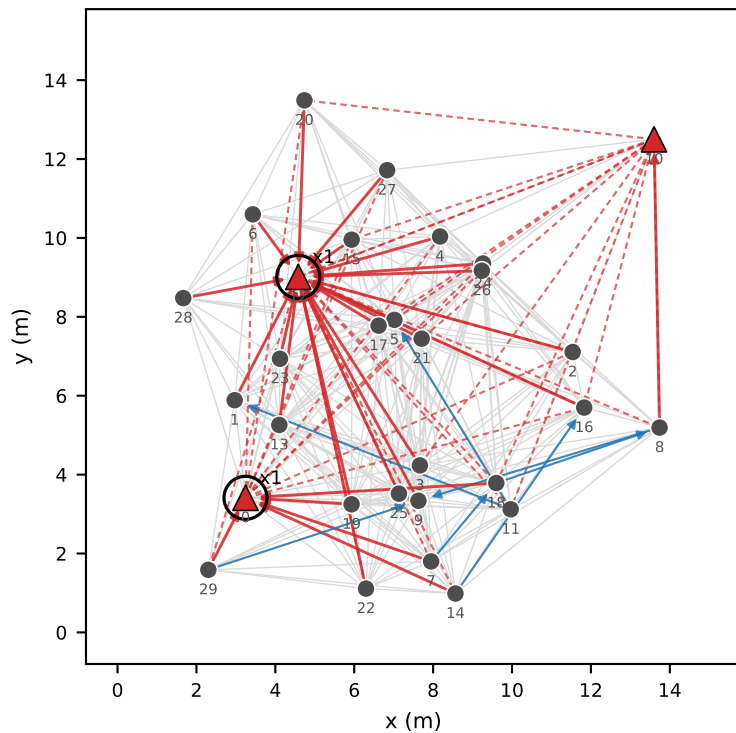
OLSR + watchdog insiders hold 79% of MPR links; honest drones excluded: 0
