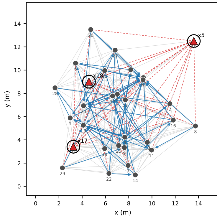
OLSR + GeoTrust+ insiders hold 0% of MPR links; honest drones excluded: 0
