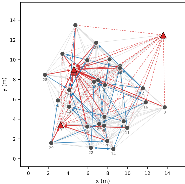
OLSR (RFC 3626) insiders hold 40% of MPR links; honest drones excluded: 0
