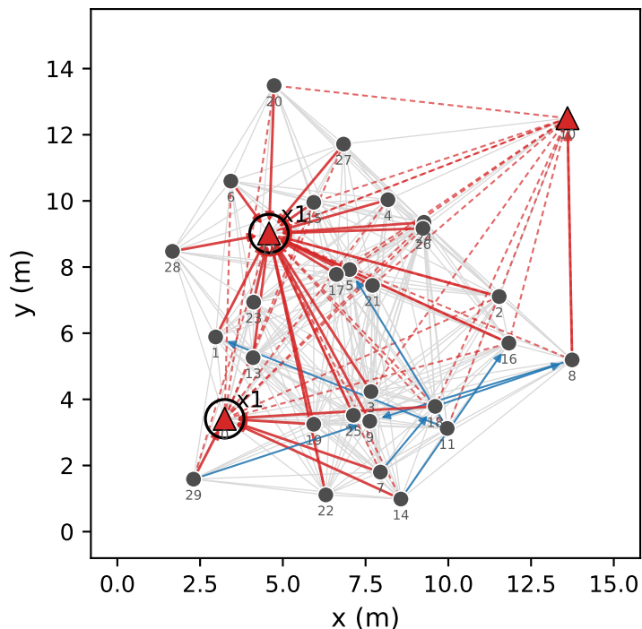
(b) OLSR + watchdog insiders hold 79% of MPR links honest drones excluded: 0
