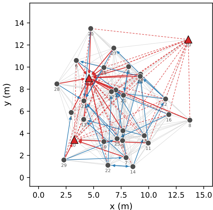
(c) OLSR + GeoTrust+ insiders hold 0% of MPR links honest drones excluded: 0
