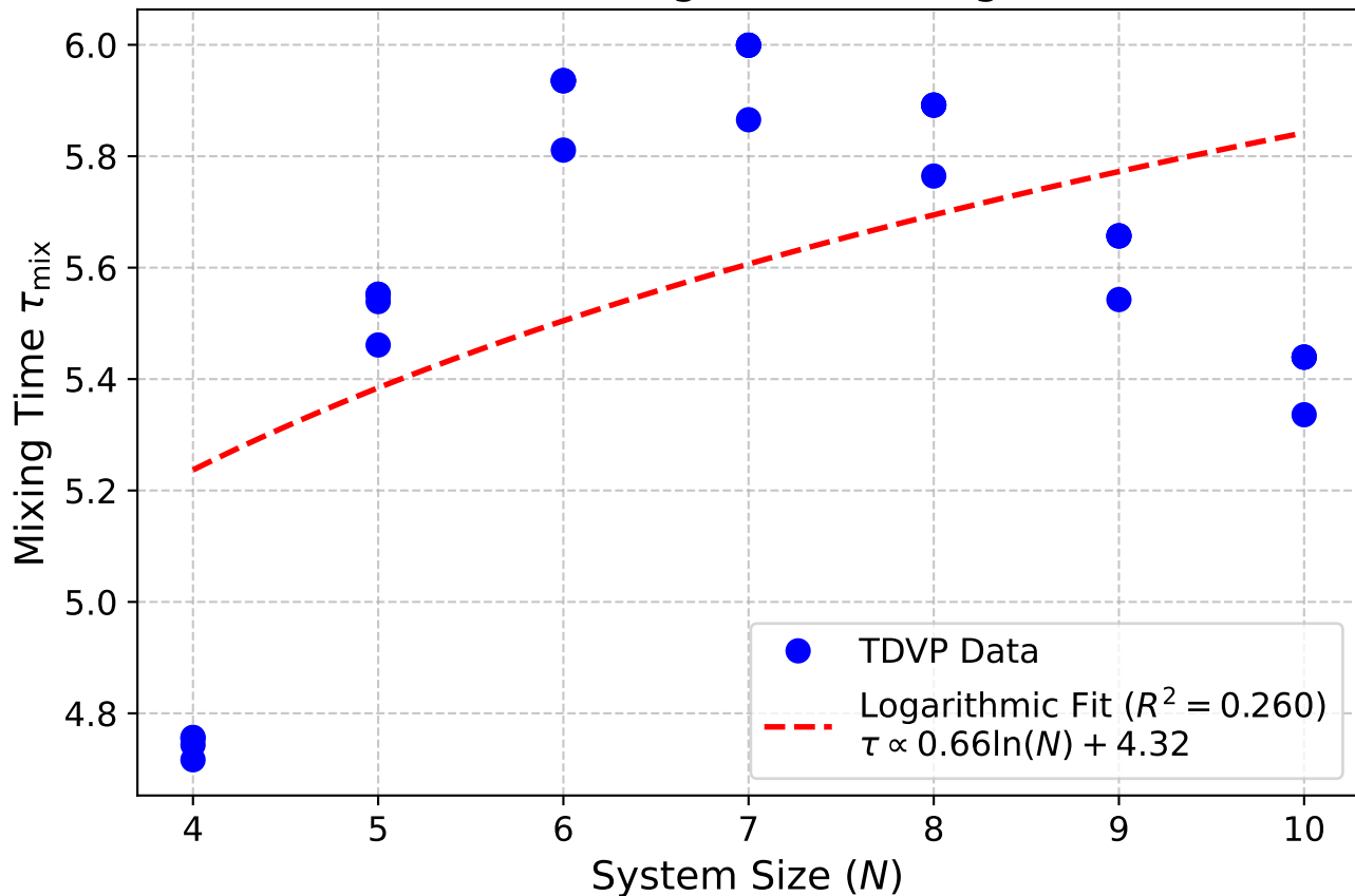
Finite-Size Scaling (Best fit: Logarithmic)
