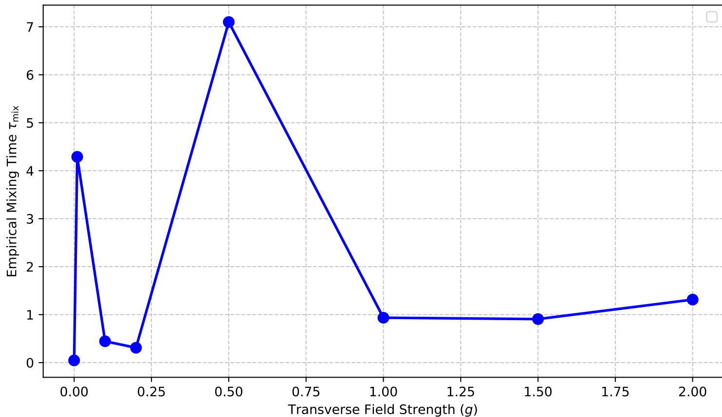
Hamiltonian-Assisted Thermalization (Pure X Bath)
