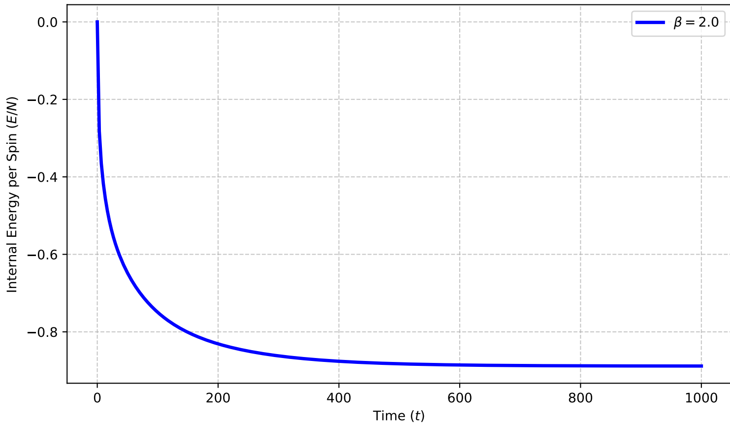
Exact Covariance Relaxation (1D TFIM, N = 6 )
