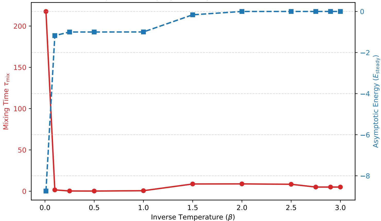
Amplitude Damping: Cooling to the Ground State
