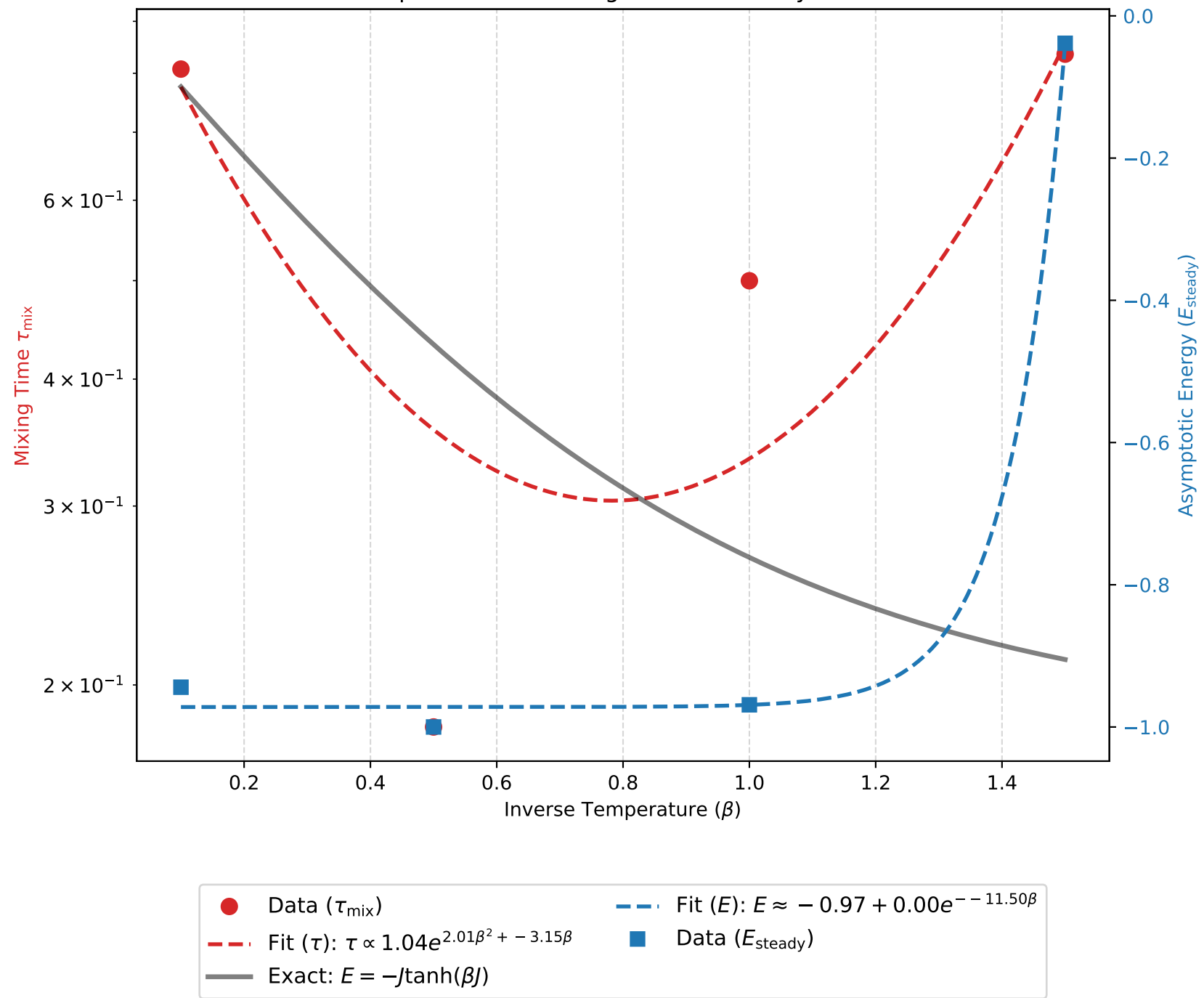
Gibbs Sampler Benchmarking: TDVP vs. Analytical Solutions
