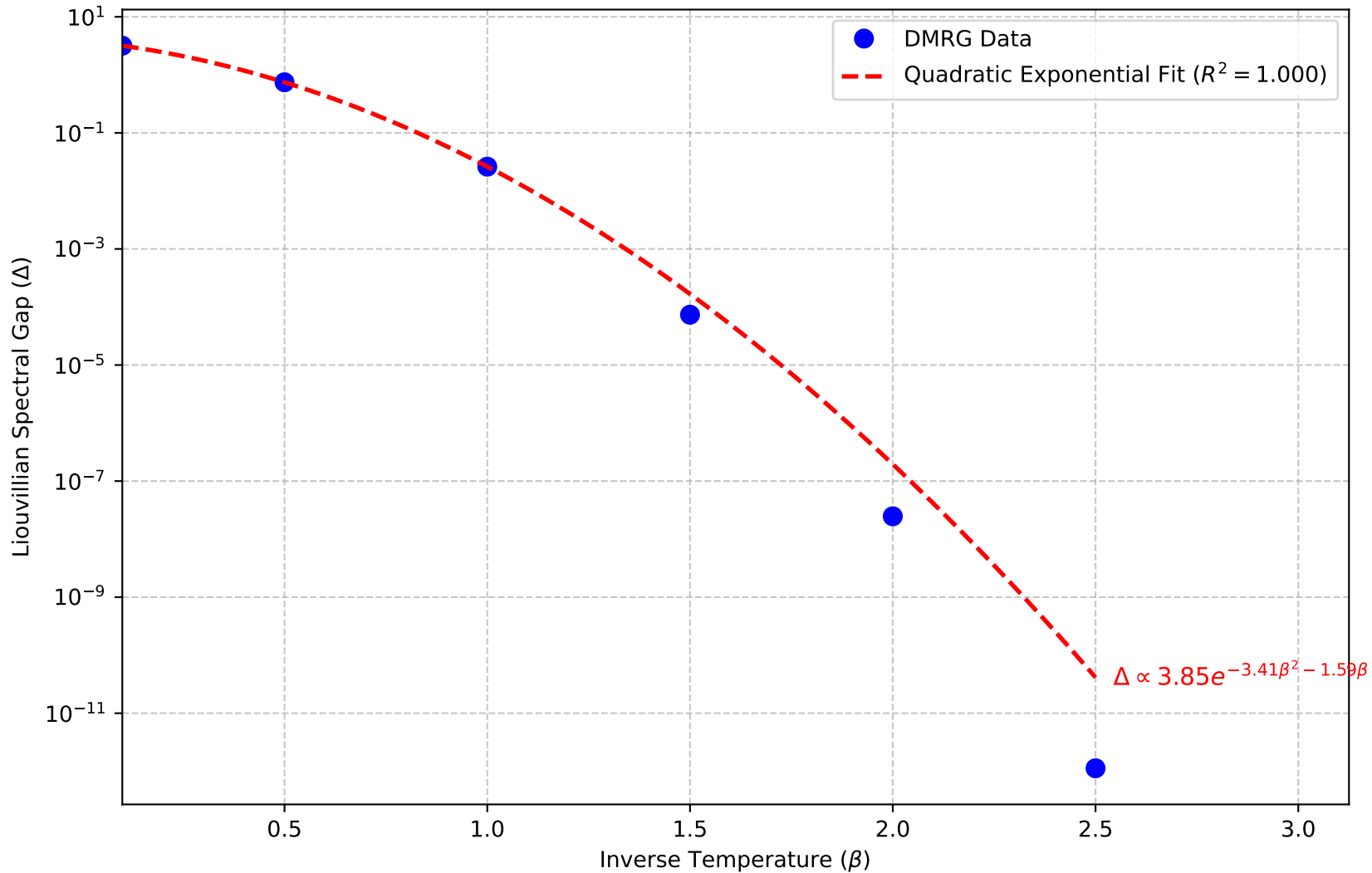
Spectral Gap vs. Inverse Temperature (1D TFIM, N = 6 )
