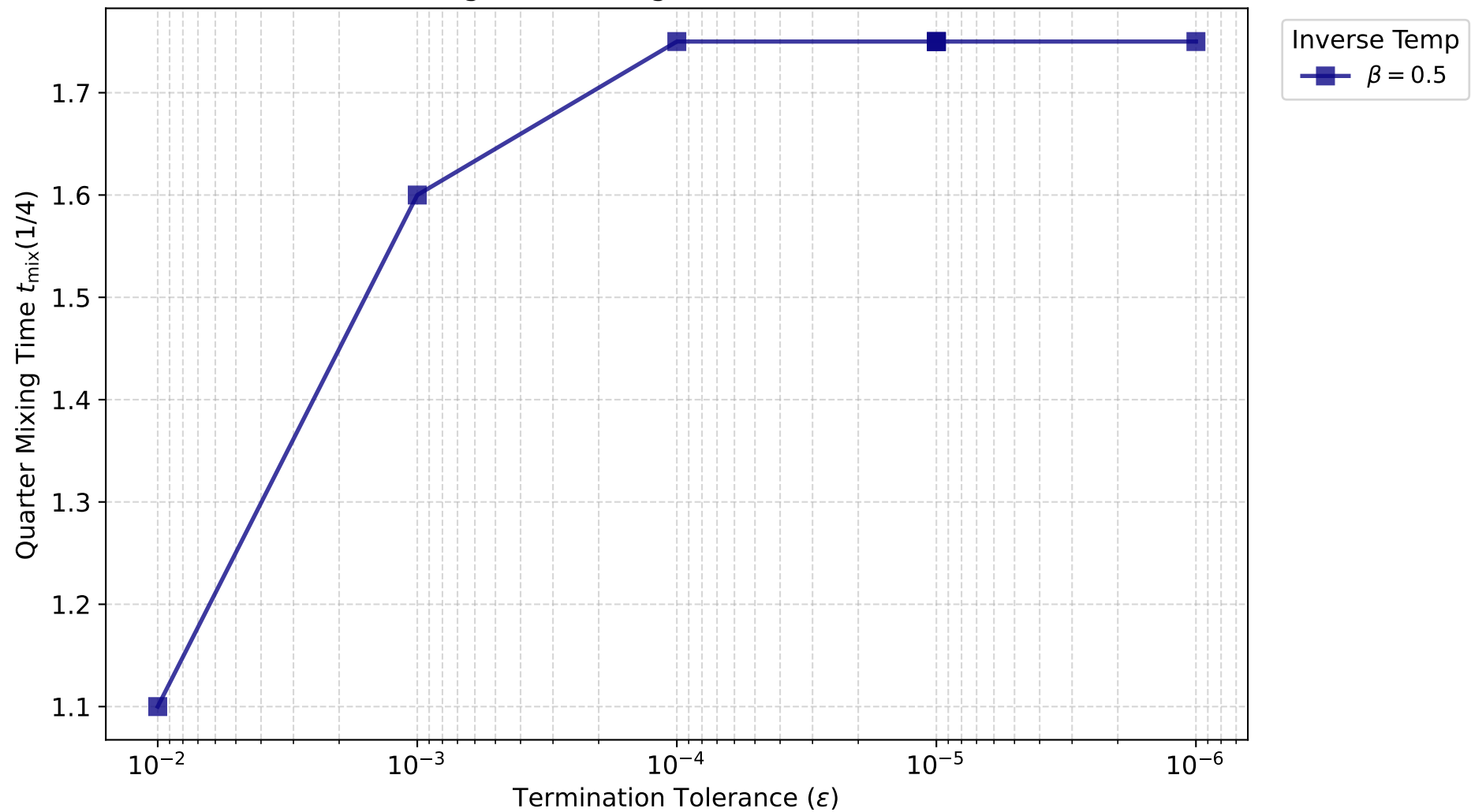
Numerical Convergence: Mixing Time vs. TDVP Tolerance ( N = 6 )
