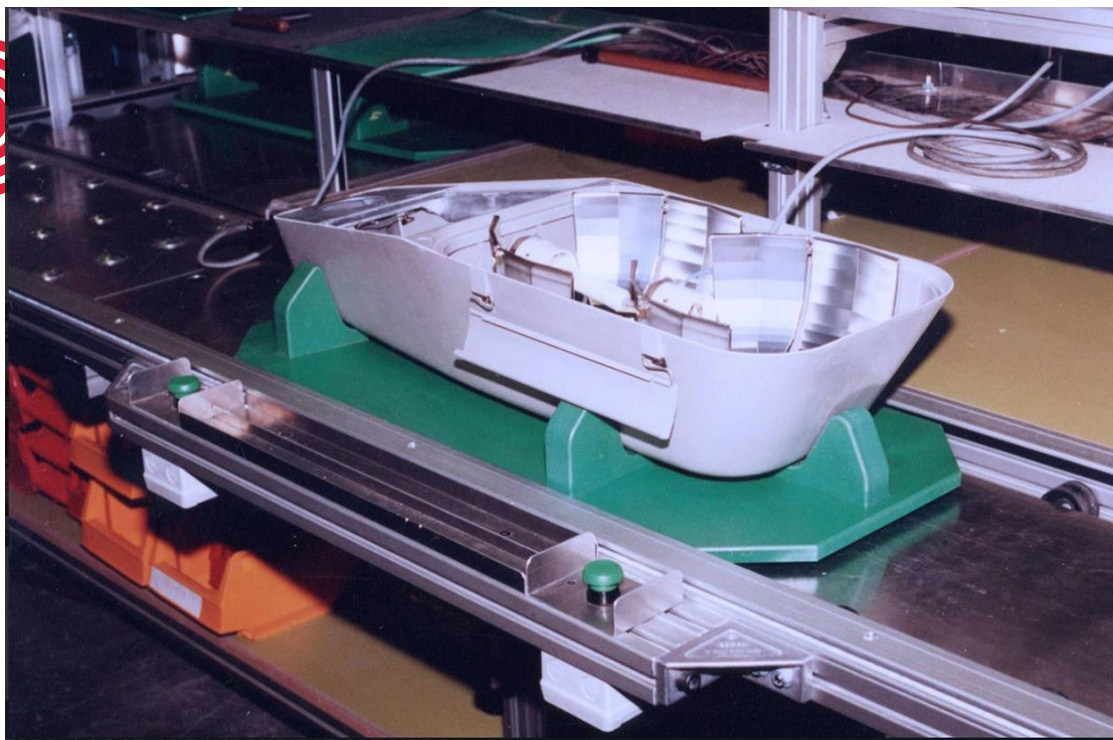
Green colored Machined pellet/Fixture/Jig/Conveyor pellet used to hold street light housing while on assembly line
