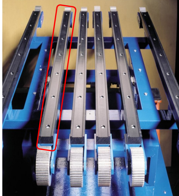
Black guides and Sprockets for small conveyors
