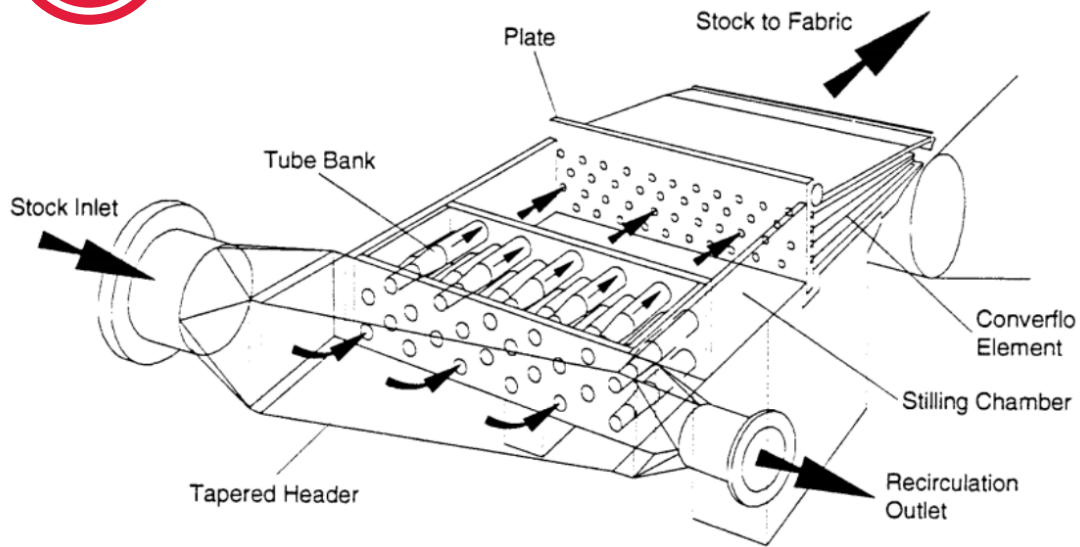
Fig 5: The plate marked in the figure above is Plascon Manifold Plate in hydraulic type headbox. Its position will vary as per design of the headbox.
