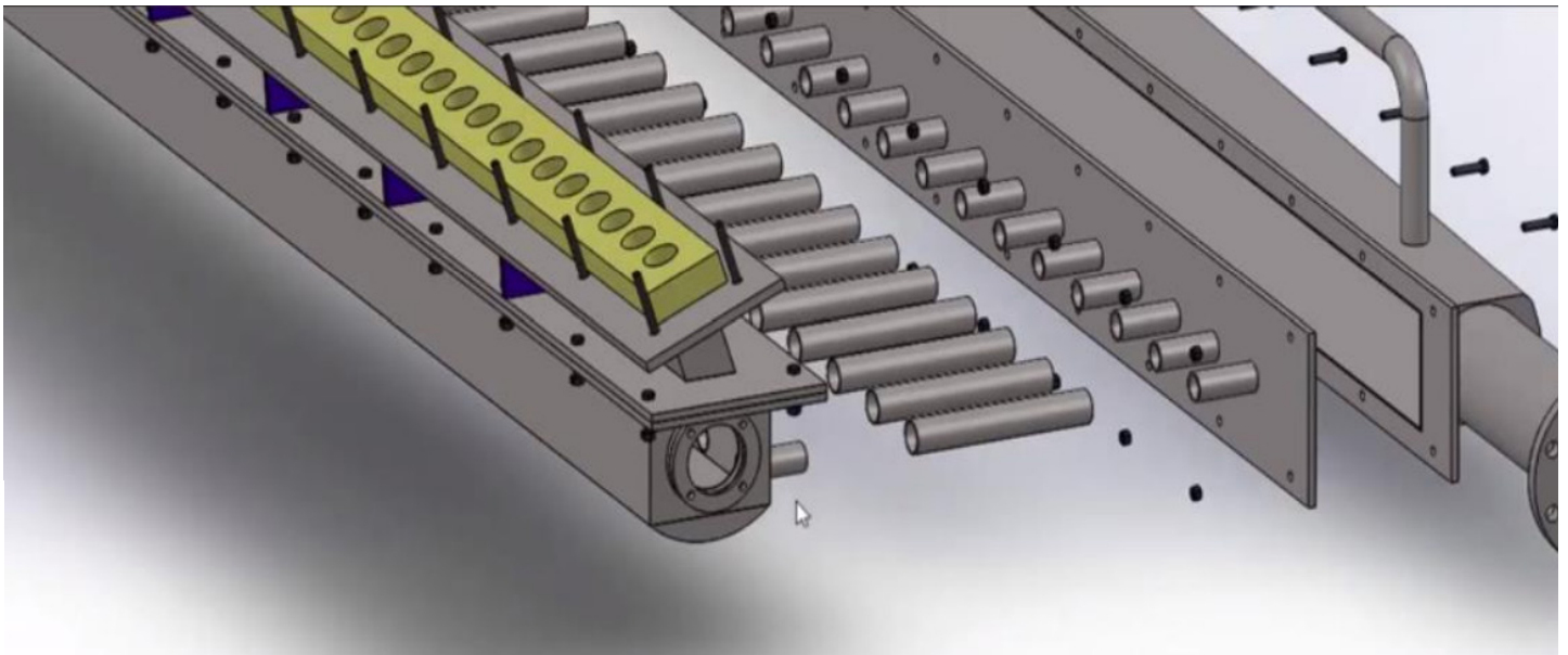
Fig 4: The yellow part is the Diffuser block/Distribution plate/ Manifold Plate, its size varies from headbox to headbox.
