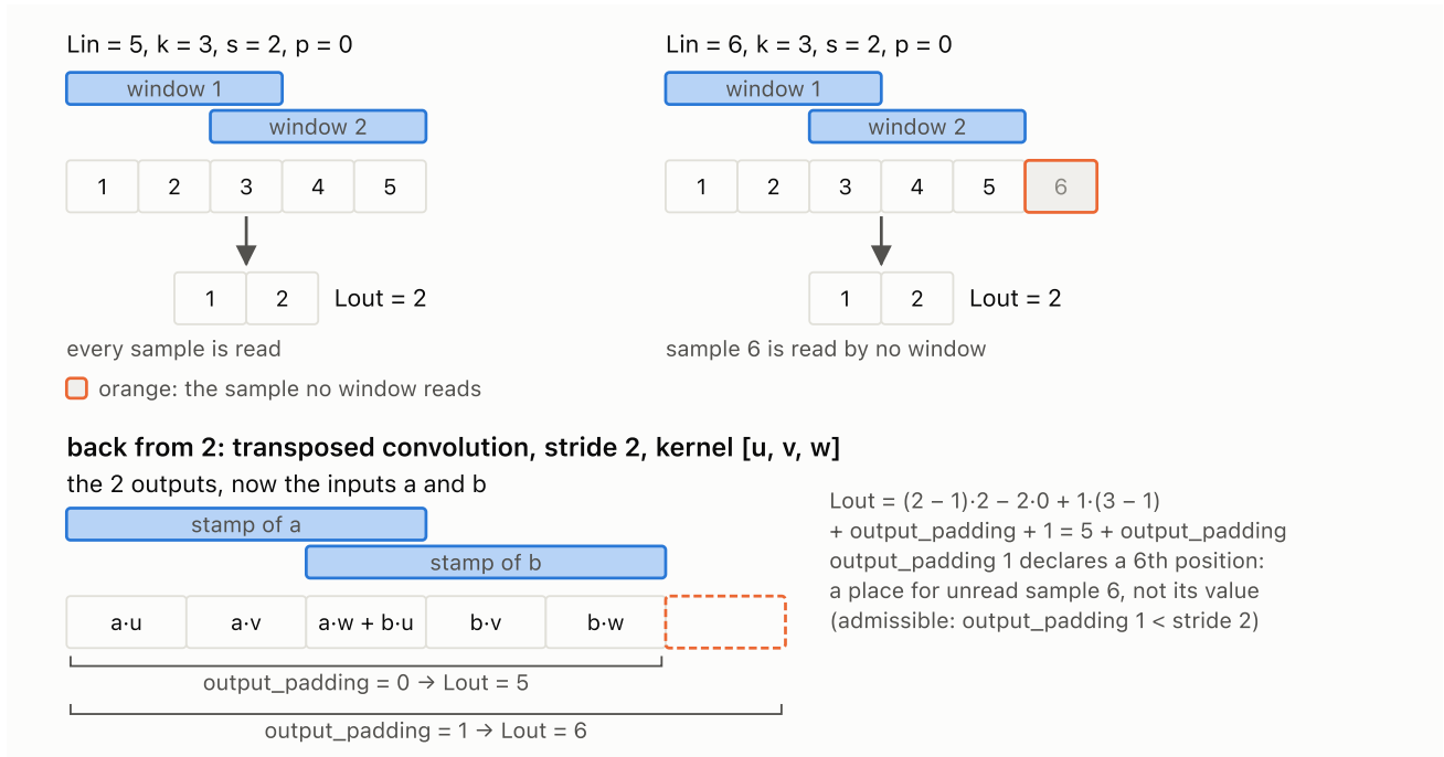
Figure 12. A forward pass with k = 3, s = 2, p = 0 reads a 5-sample and a 6-sample conveyor signal with the same two windows, so both give L_{out} = 2 and the sixth sample is never read; going back from 2, the two stamps cover five positions, and \text{output\_padding} = 1 only declares a sixth so that L_{out} is 6 again; the value of the sample the forward pass never read is not restored.
