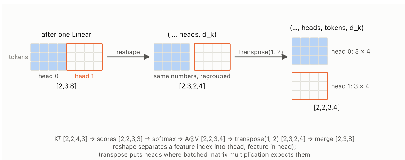
Figure 20. The shape walk for B=2 , T=3 , D=8 , H=2 : reshape separates each projected feature index into (head, feature within head), [2, 3, 8] \rightarrow [2, 3, 2, 4]; transpose(1, 2) puts heads where batched matrix multiplication expects them, [2, 2, 3, 4]; and the inverse pair after A @ V restores [2, 3, 8] with the token order intact.
