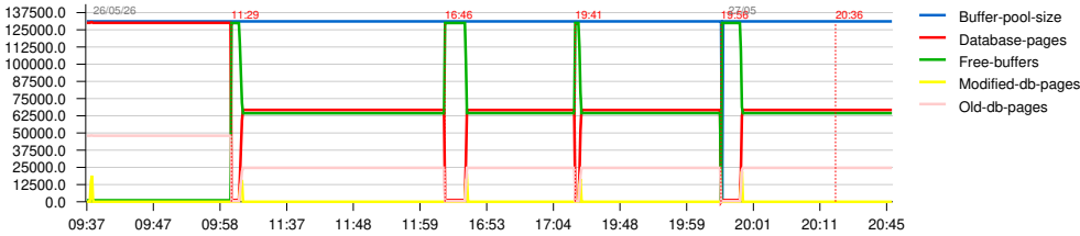
InnoDB Buffer Pool Usage: point-select,6 core: bare metal/ k8 port-forward+docker/ k8 Nodeport+docker / k8 LB +docker/ k8 Nodeport+ containerd - [Value]
