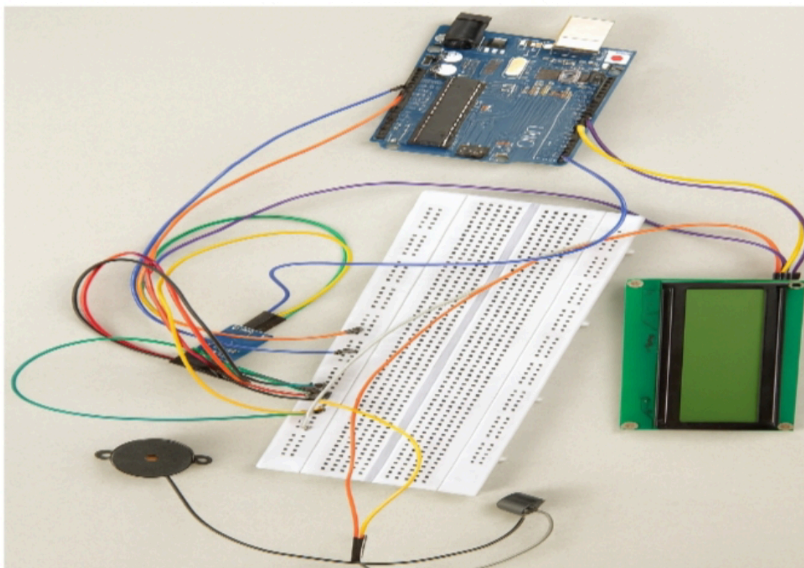
Fig 3.2-Manual Connection
