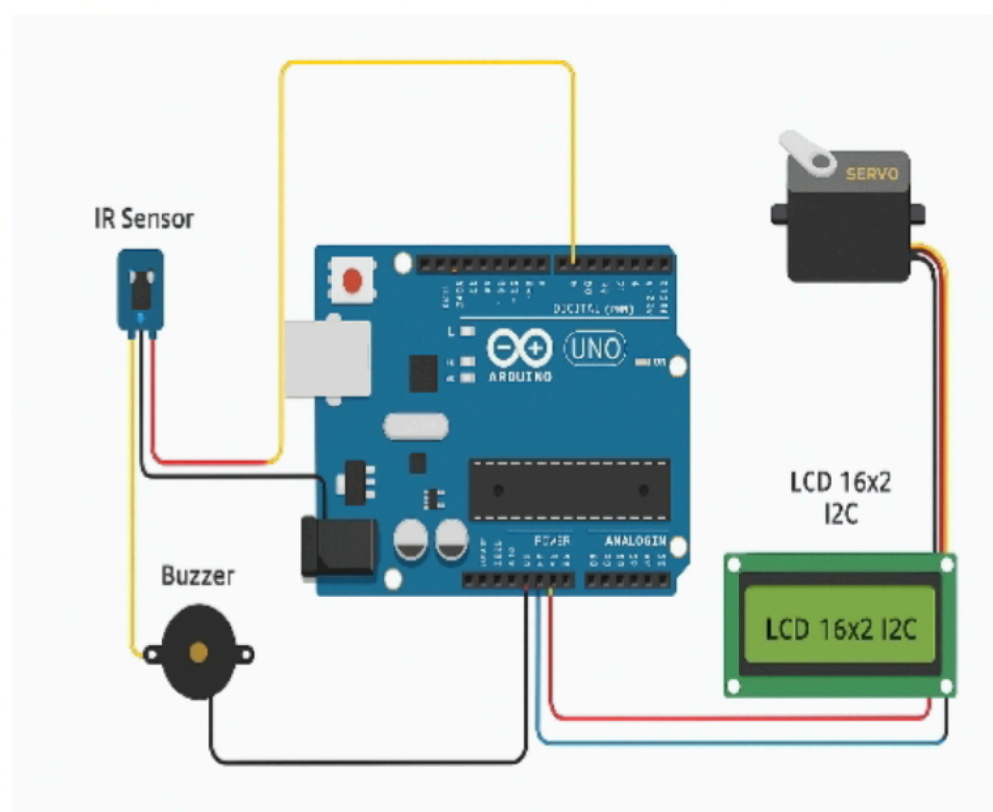
Fig-3.1 PIN OUT DIAGRAM
