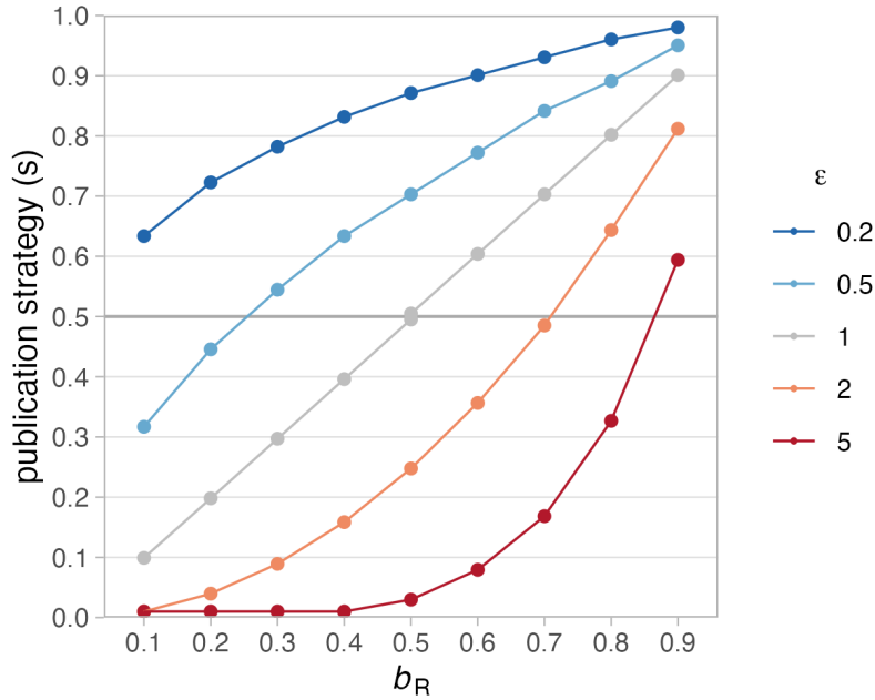
Figure A1: Effect of fitness functions on publication strategies. Shown are publication strategies ( s ) that maximise expected fitness for different fitness functions, with one research cycle per generation ( m = 1 ), no survival threshold ( \delta = 0 ) and no competition ( \gamma = 1 ). Fitness functions with \epsilon = 0.2 and \epsilon = 0.5 (blue lines) are concave with diminishing returns, functions with \epsilon = 2 and \epsilon = 5 (red lines) are convex with increasing returns; the function with \epsilon = 1 (grey line) is linear.
