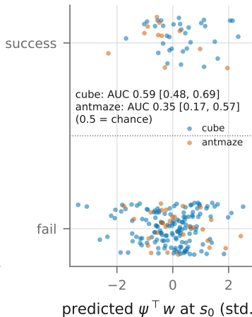
(c) does the value predict the outcome?
