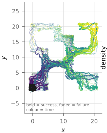
(a) antmaze rollouts 11/40 reach the goal
