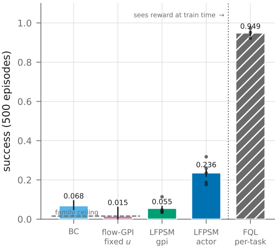
(a) cube-single, Wilson 95% intervals
