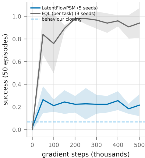
(b) training curves, mean \pm 95% CI
