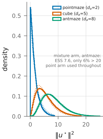
(b) inverted latents are typical (dotted: \chi^2_{d_a} )
