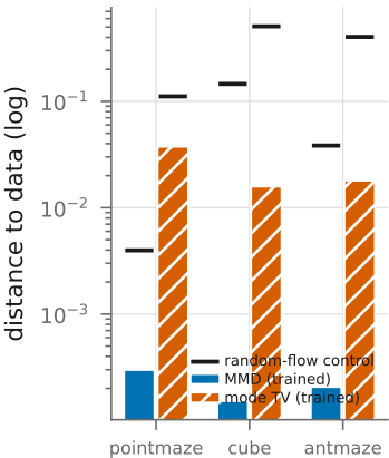
(a) flow vs a random-flow control
