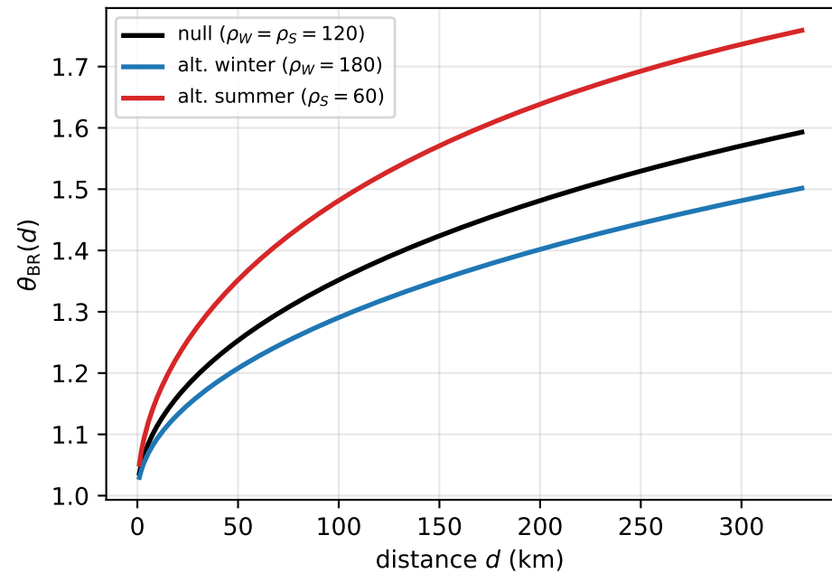
Extremal coefficient
