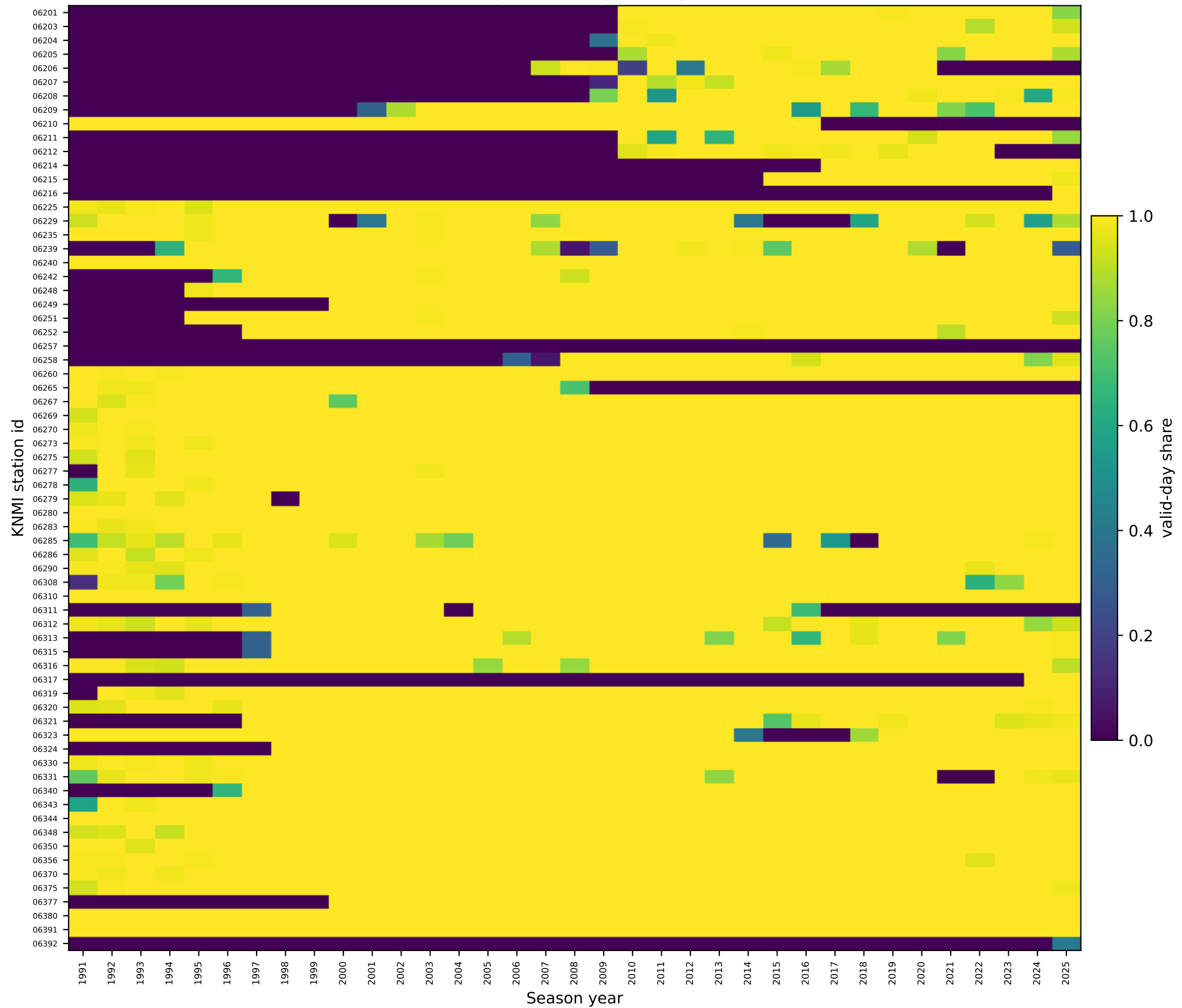
Daily maximum FX coverage: valid-day share per station-season (DJF)
