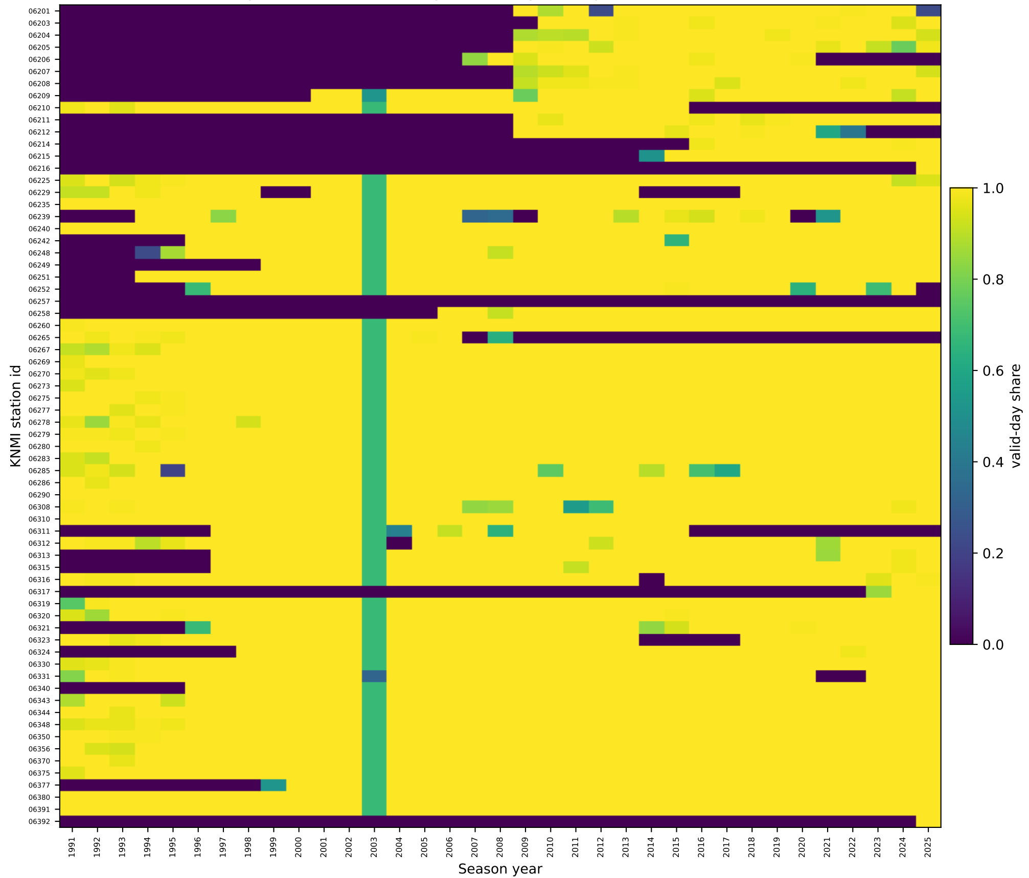
Daily maximum FX coverage: valid-day share per station-season (JJA)
