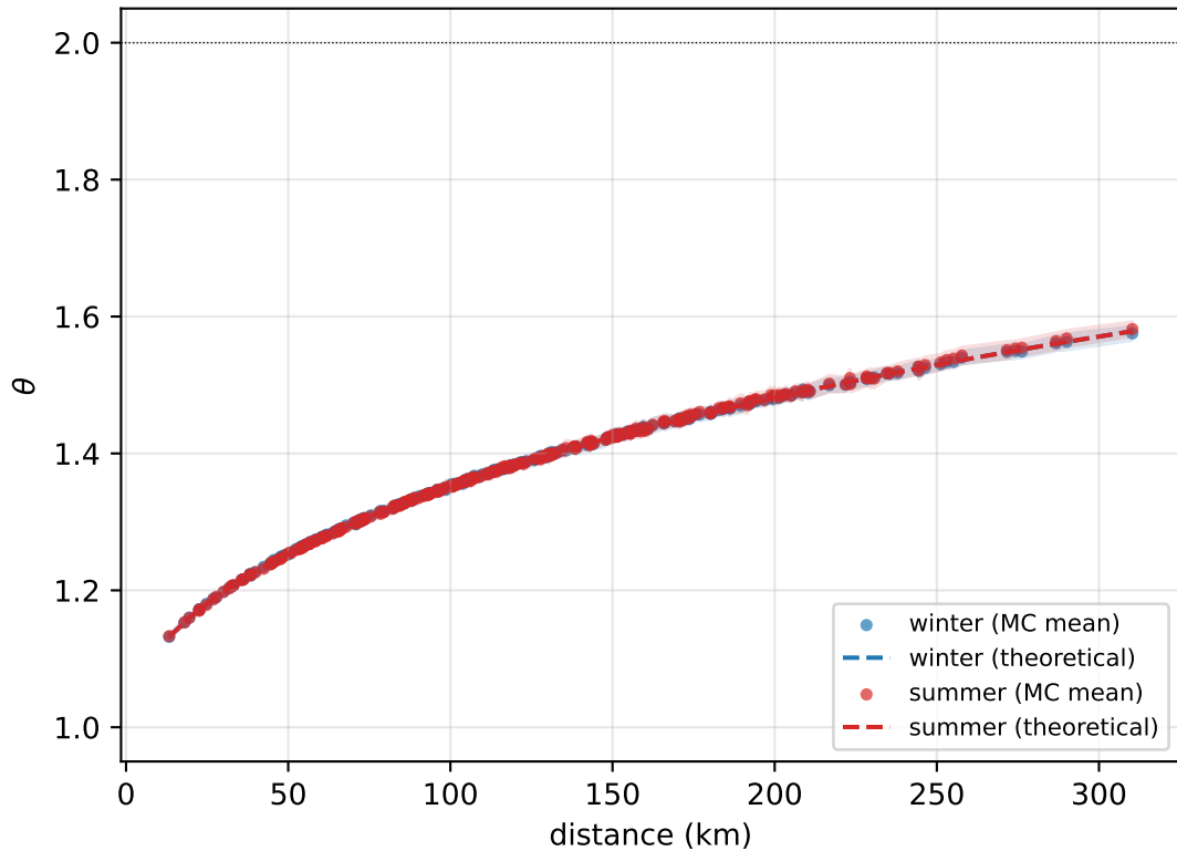
Estimated theta vs distance (null)
