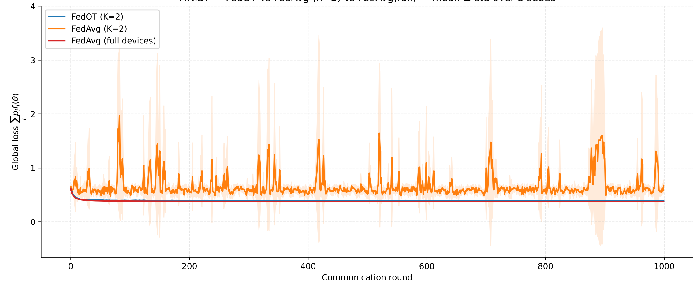
MNIST — FedOT vs FedAvg (K=2) vs FedAvg(full) — mean \pm std over 5 seeds
