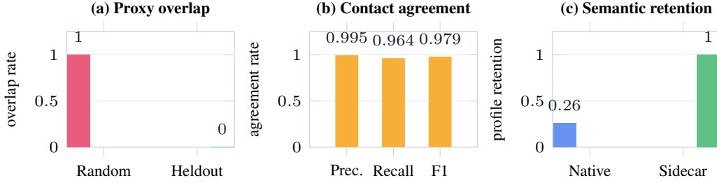
Figure 2: Summary of the displayed audits. Proxy overlap is confounded with task holdout; contact agreement pools 32 paired scenarios; sidecar retention is by construction.
