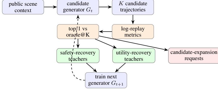
Figure 1: REGRETBOT separates candidate-generation failure from recoverable selection regret. Safety and utility cases produce in-bank teacher trajectories for bootstrapping. Generation-gap cases do not: they request a richer candidate distribution.
