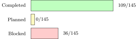
Fig. 3. Configured CVM status. The denominator is 145 configured rows; planned rows, if any, are not launched, and blocked rows name true precondition or ablation-support gaps.
