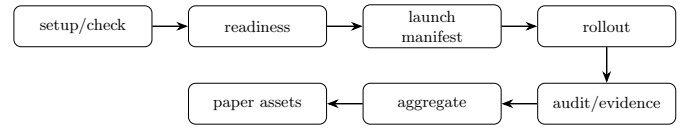
Fig. 2. The contract-validation pipeline separates setup, readiness, manifest materialization, rollout, audit, aggregation, and paper-asset generation.
