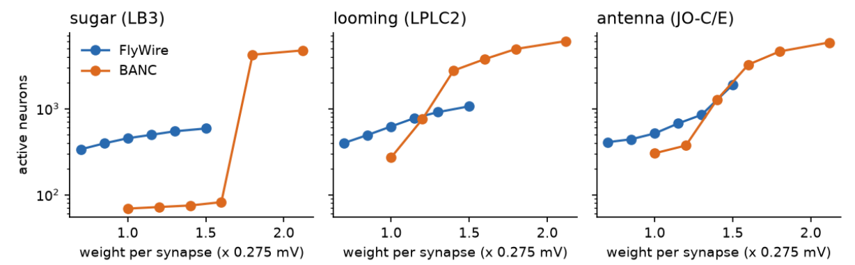
Figure 3. Active neurons as the weight per synapse is scaled, in FlyWire and in BANC (v2), for three stimuli.
