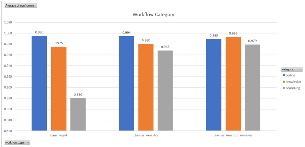
Figure 2. Workflow performance across task categories.
