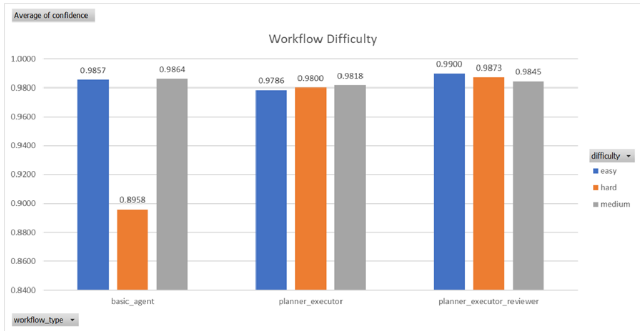
Figure 3. Workflow performance across difficulty levels.
