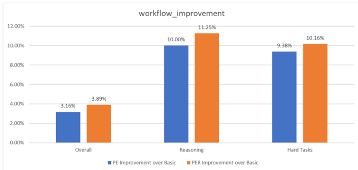
Figure 4. Percentage improvement relative to the Basic Agent baseline.
