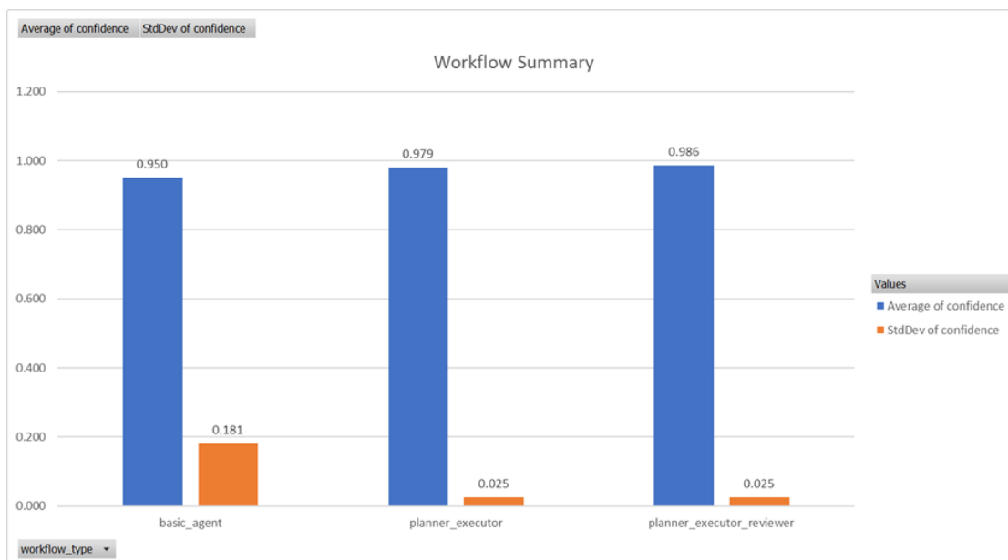
Figure 1. Average confidence and standard deviation across workflow architectures.
