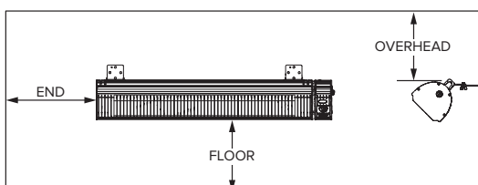
Clearances
