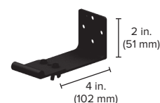
Mounting Bracket 4
