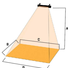
Heating Coverage
