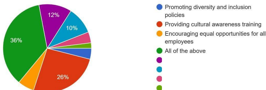
Fig 10: Perceived Effectiveness of Specific HR Roles
