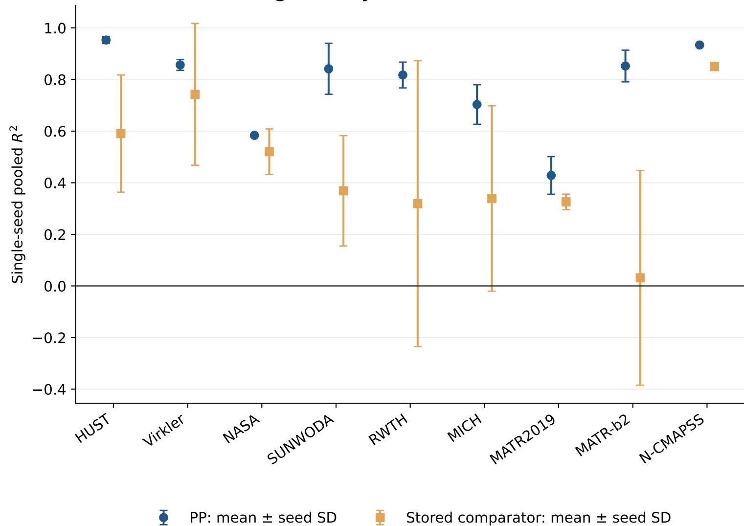
Retraining stability across five matched seeds
