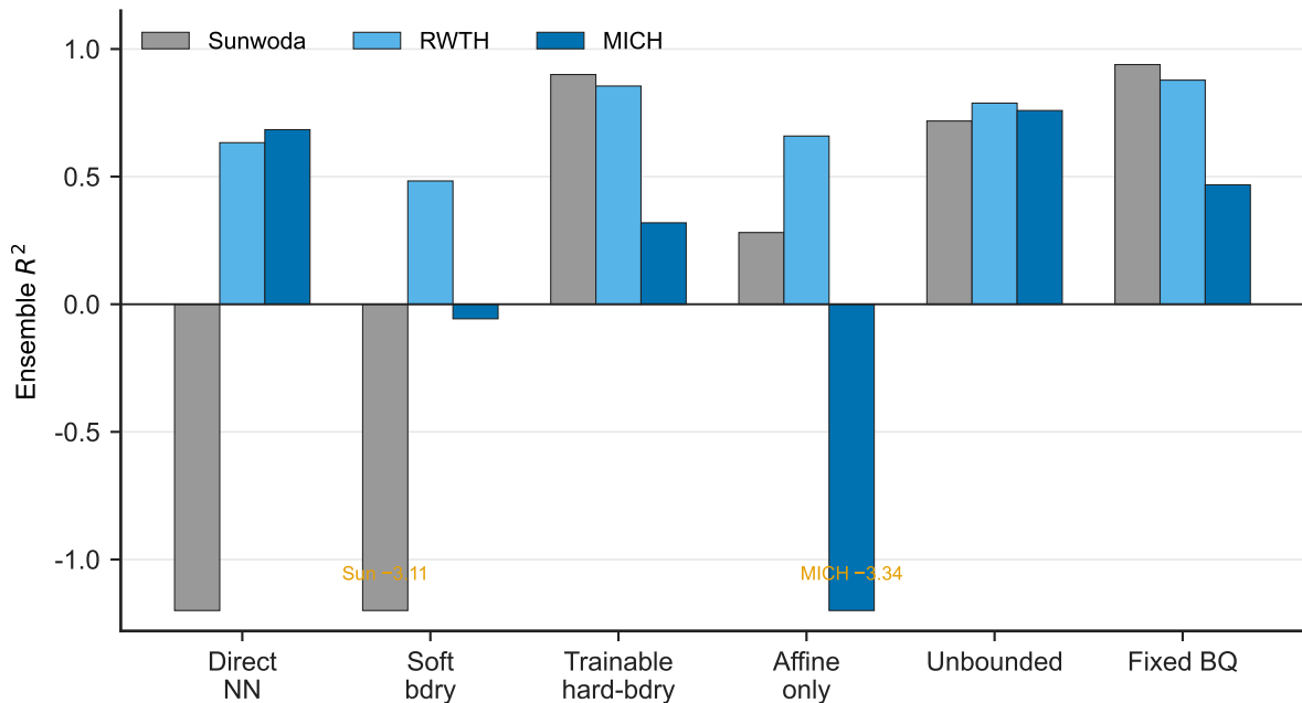
Matched 6-arm ablation (ensemble R^2 )
