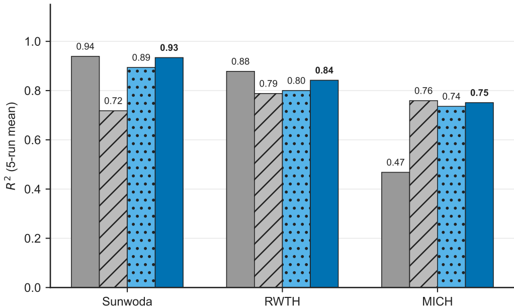
Development results (3 datasets) Fixed bound Unbounded Distance SAAR
