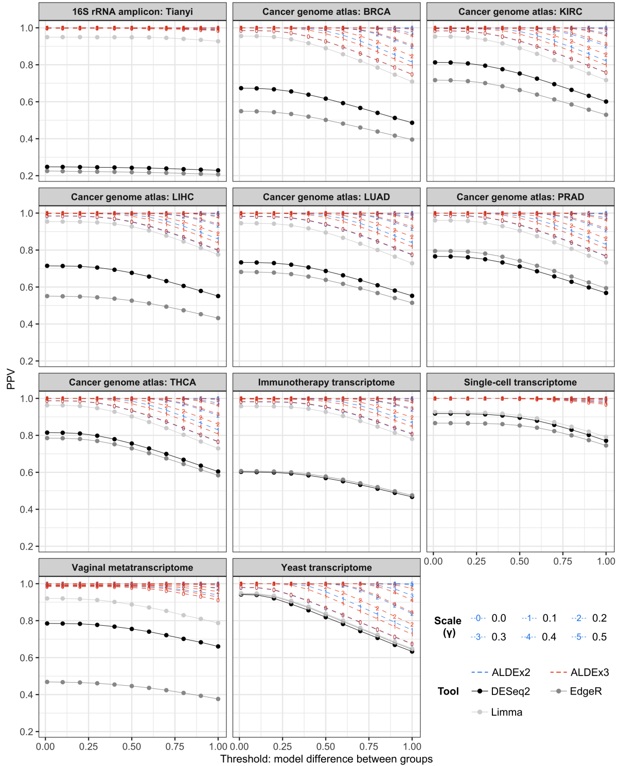
Supplementary Figure S2: Positive predictive values for all datasets tested. The positive predictive value (PPV) for all tool and dataset combinations was calculated separately for each 0.1 increment in the model difference between groups (i.e. the simulated or ‘true’ \log_2 fold-change between groups, as determined by binomial thinning). Each data point represents the PPV when considering dataset features with a simulated log-difference at or above the given x-axis threshold. Features were considered differentially abundant at a BH-adjusted P -value of <0.05 .
