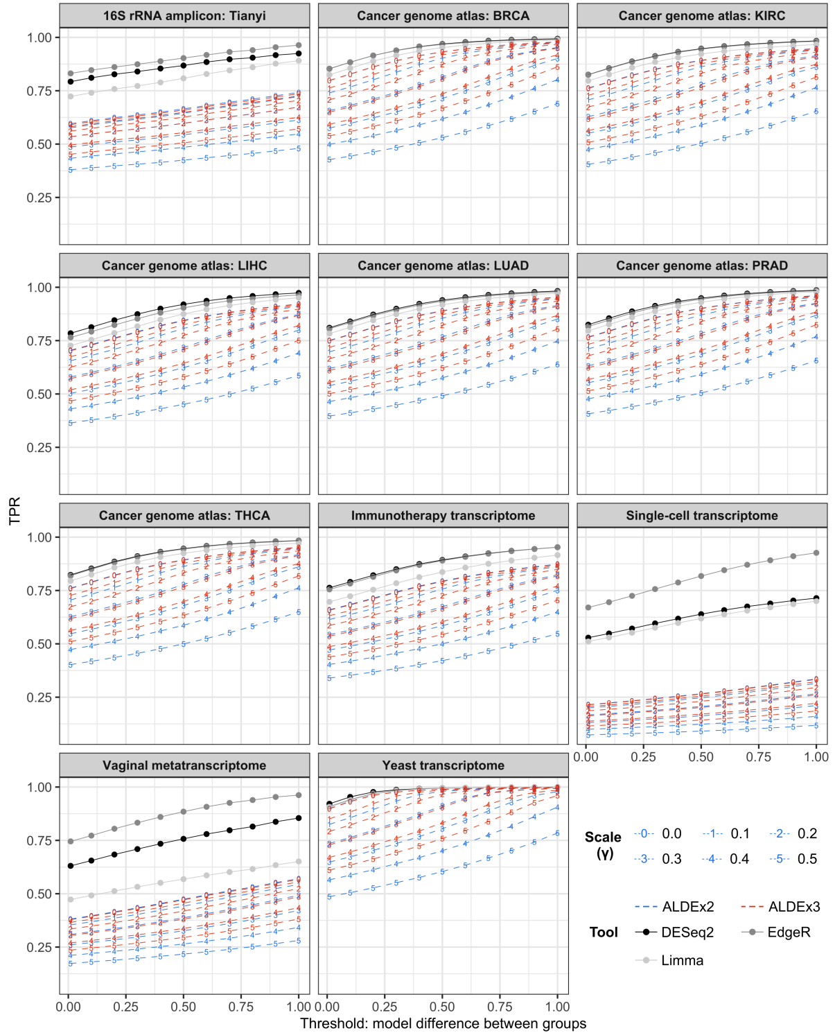
Supplementary Figure S3: True-positive rates for all datasets tested. True positive rates (TPR) for all tool and dataset combinations were calculated separately for each 0.1 increment in the model difference between groups (i.e. the simulated or ‘true’ \log_2 fold-change between groups, as determined by binomial thinning). Each data point represents the TPR when considering dataset features with a simulated log-difference at or above the given x-axis threshold. Features were considered differentially abundant at a BH-adjusted P -value of <0.05 .
