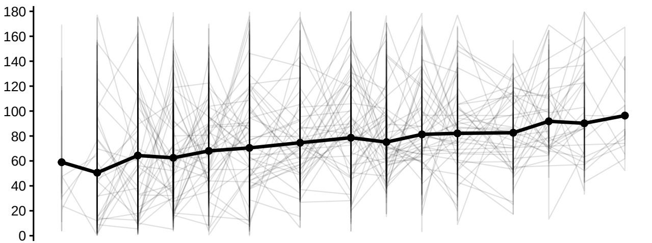
NN1
