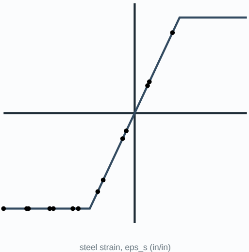
Steel stress-strain
