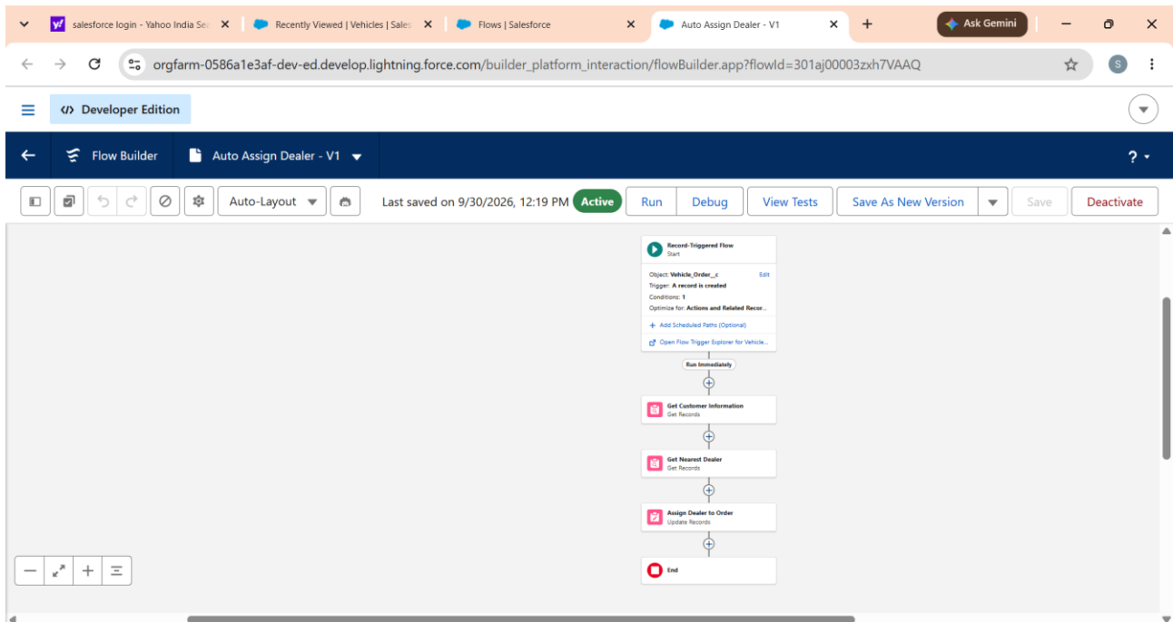
Screenshot 5.3: Auto Assign Dealer Flow- Flow canvas with Get Customer Information, Get Nearest Dealer and Assign Dealer to Order elements.
