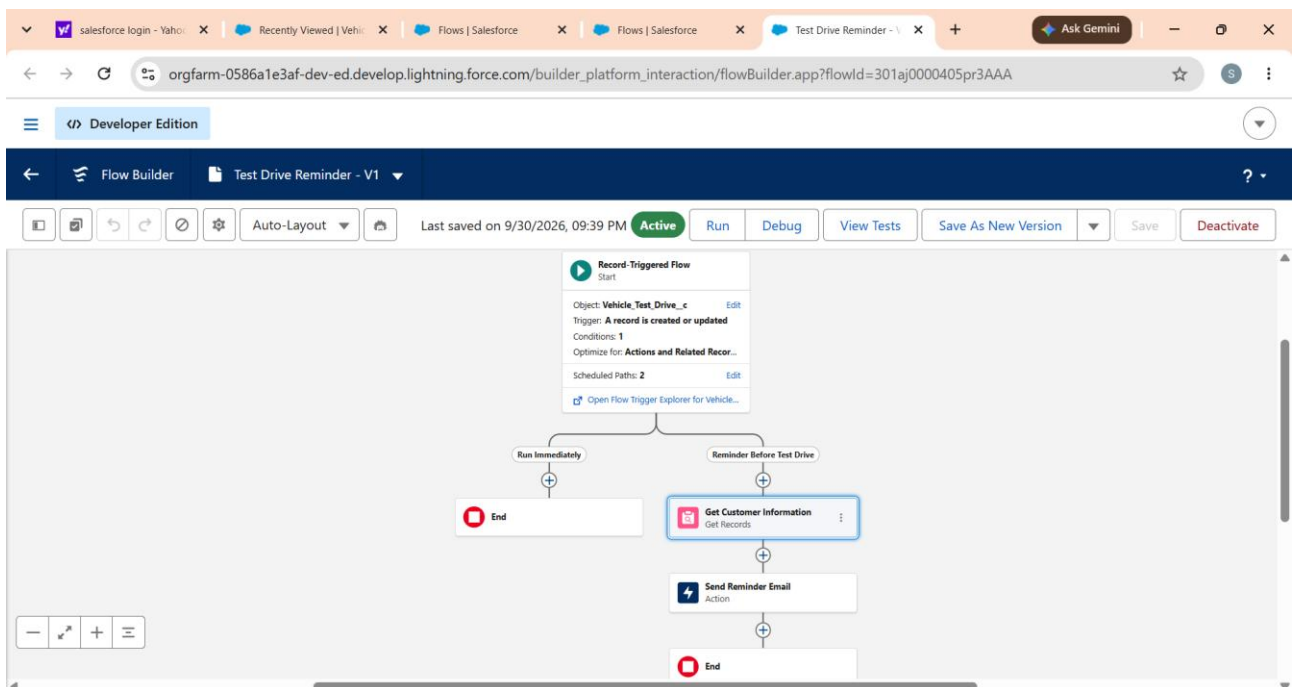
Screenshot 5.4: Test Drive Reminder Flow - Scheduled path (1 day before), Get Records and Send Email action.
