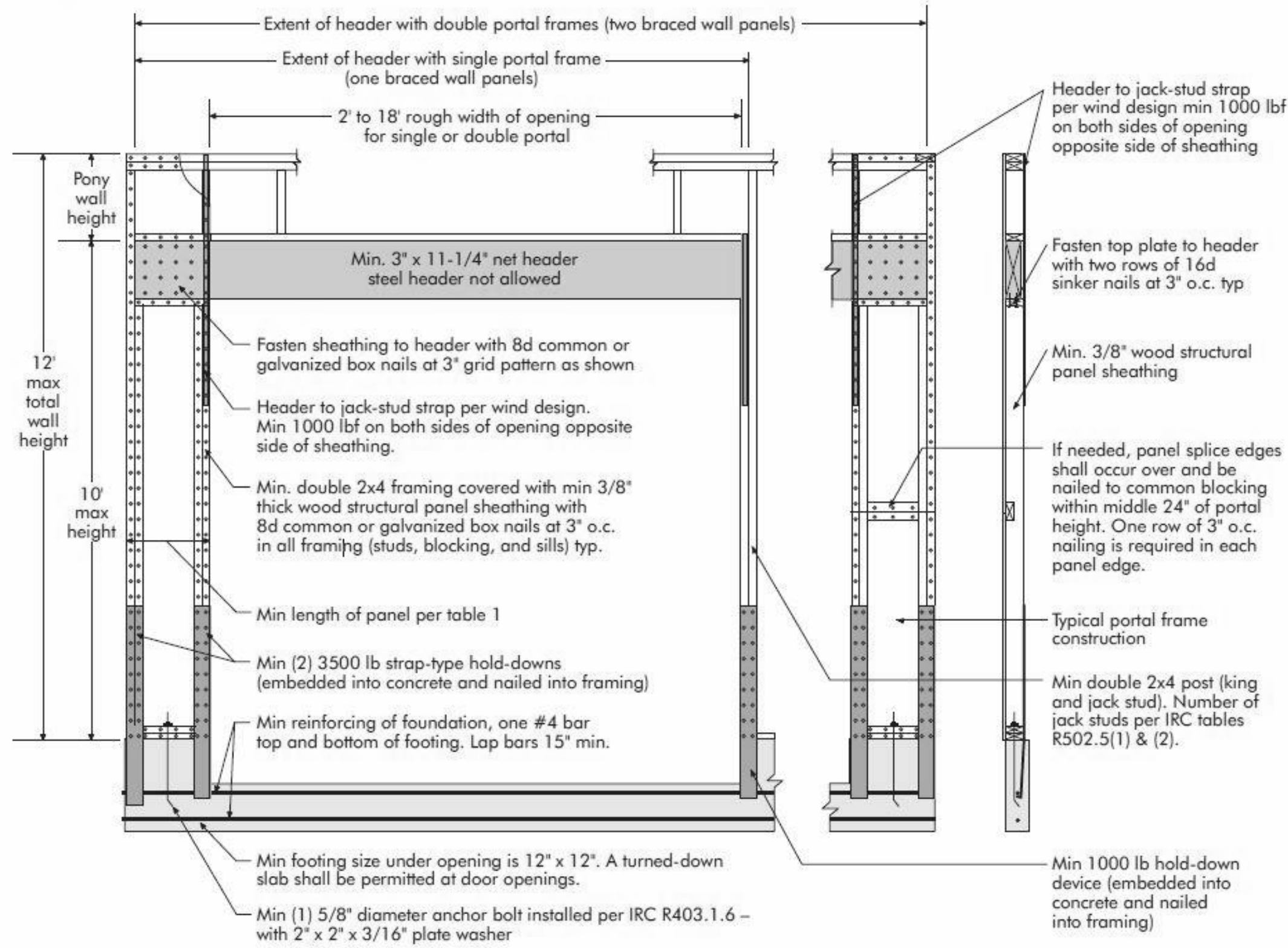
1 APA PORTAL-FRAME DETAIL 1/4" = 1'-0"
