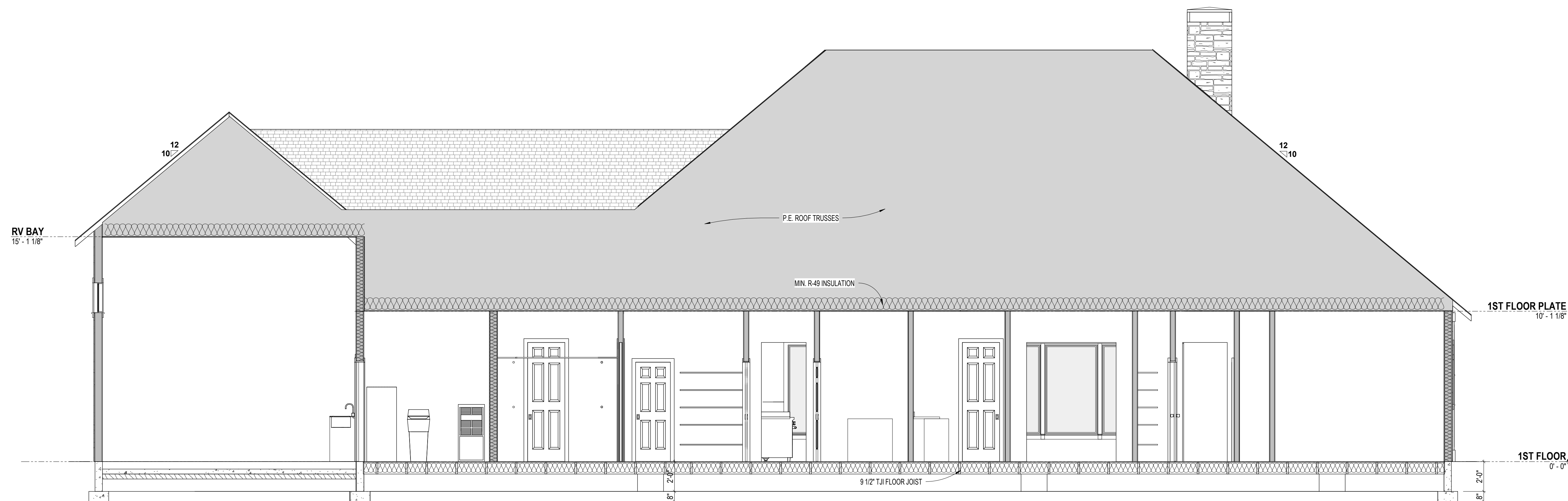
1 BUILDING SECTION-1 1/4" = 1'-0"
