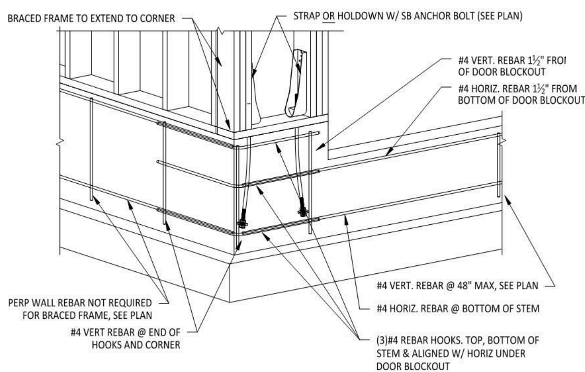
2 S1.1 ENG. BRACE FRAME SCALE: 3/4" = 1'-0"
