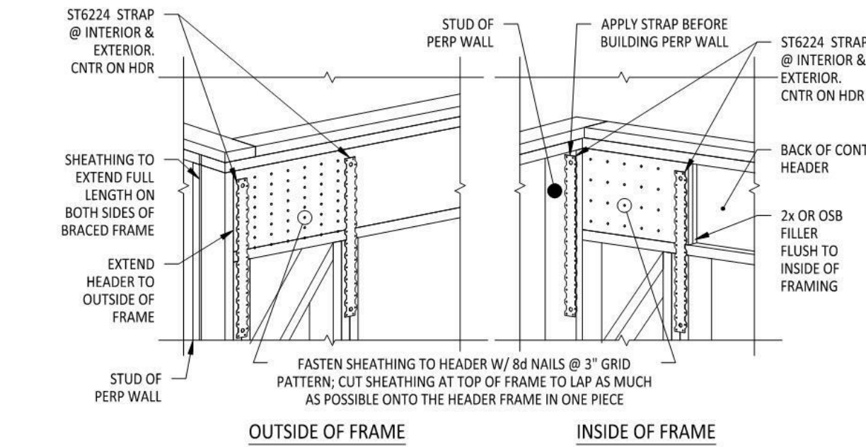
4 S1.1 ENG. BRACE FRAME SCALE: 3/4" = 1'-0"
