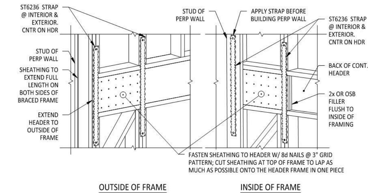
3 S1.1 ENG. BRACE FRAME SCALE: 3/4" = 1'-0"
