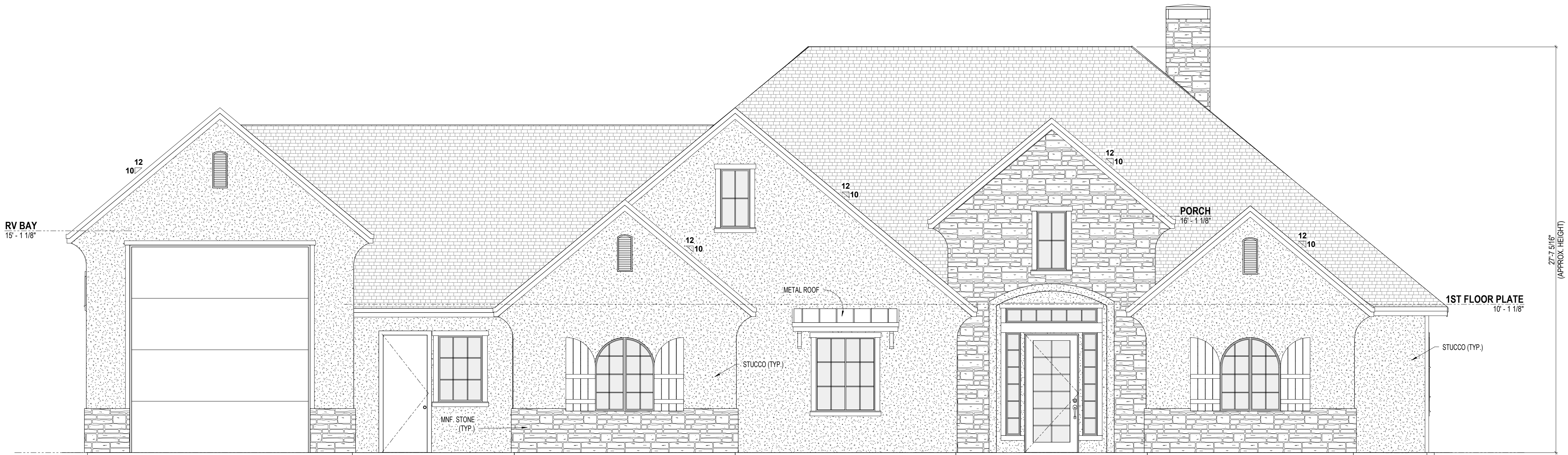
1 FRONT VIEW 1/4" = 1'-0"
