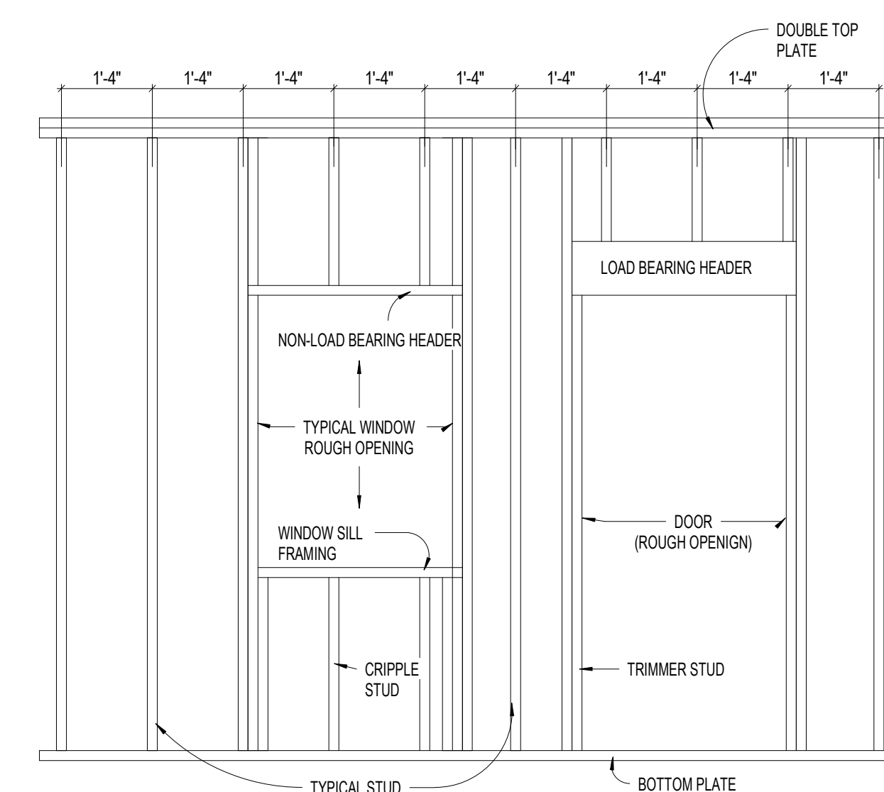
3 FRAMING DETAIL 1/2" = 1'-0"
