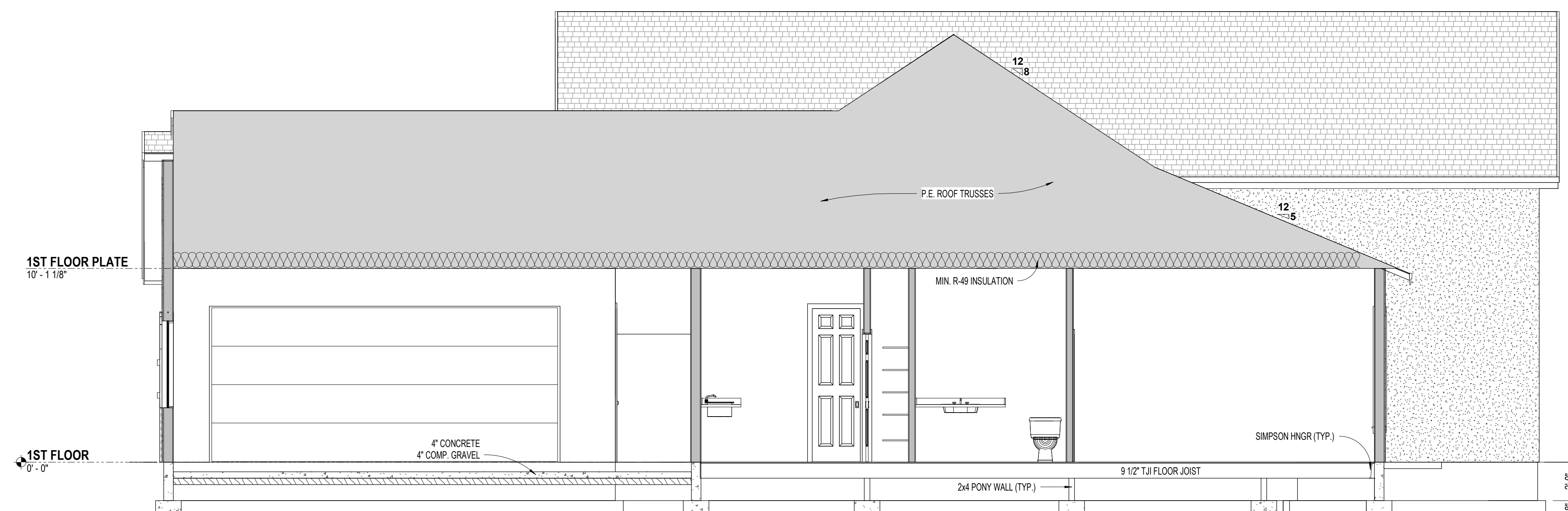
2 BUILDING SECTION-2 1/4" = 1'-0"
