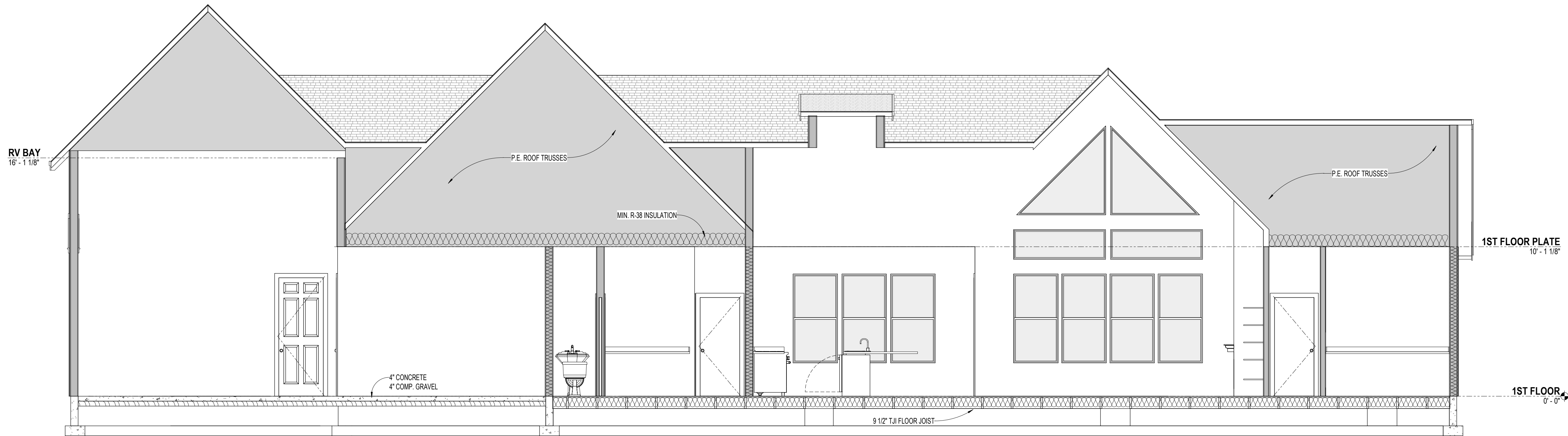
2 BUILDING SECTION-2 1/4" = 1'-0"
