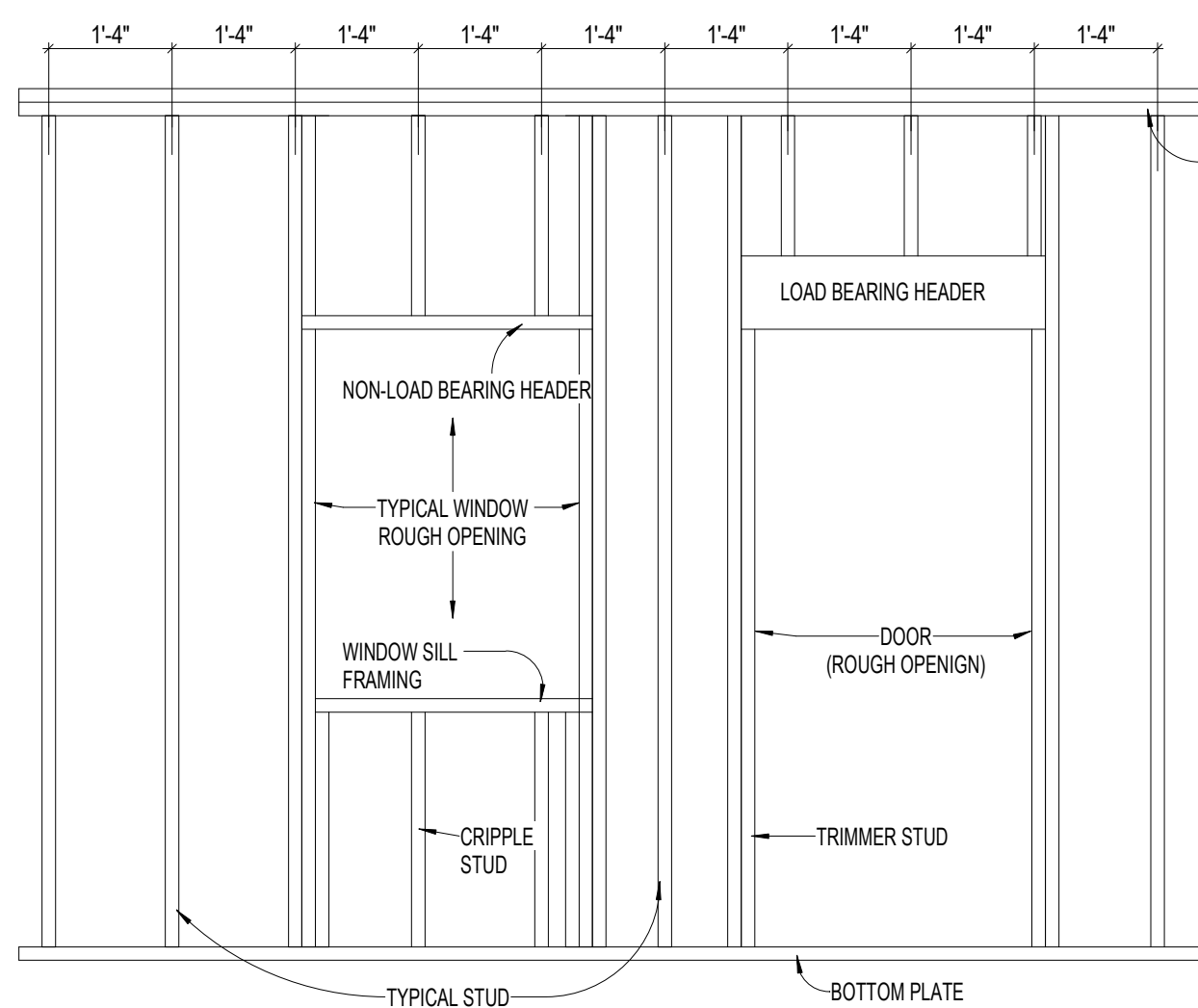
2 FRAMING DETAIL 1/2" = 1'-0"
