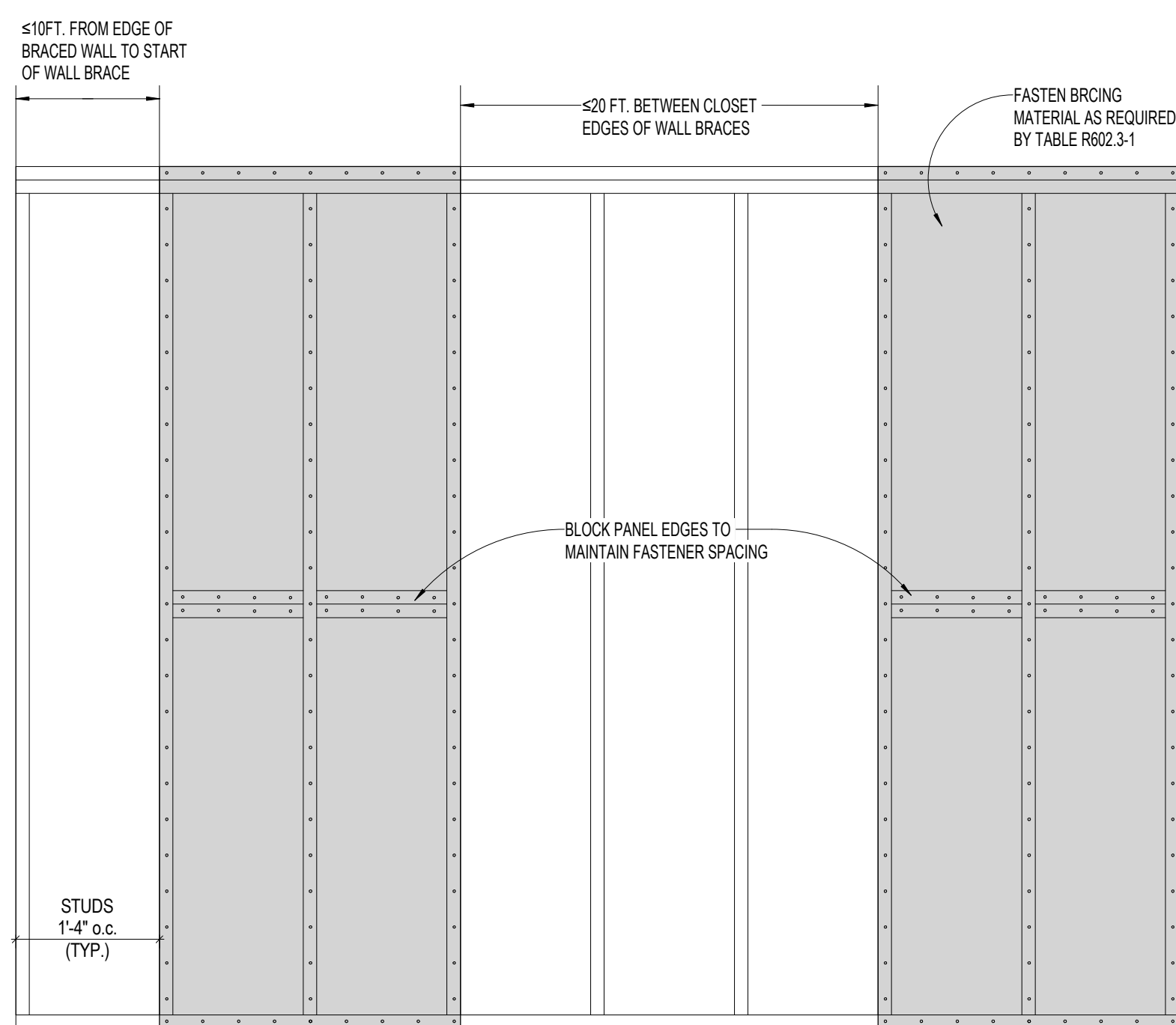
5 WSP DETAIL 3/4" = 1'-0"
