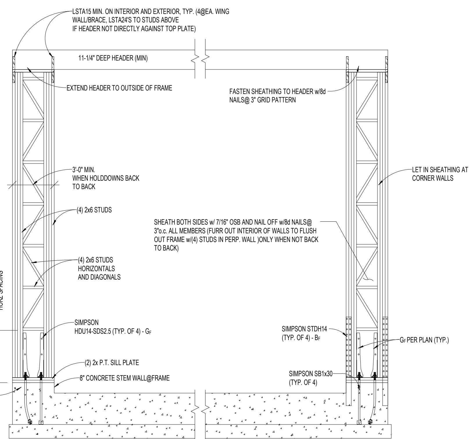
6 PORTAL FRAME DETAIL 3/8" = 1'-0"
