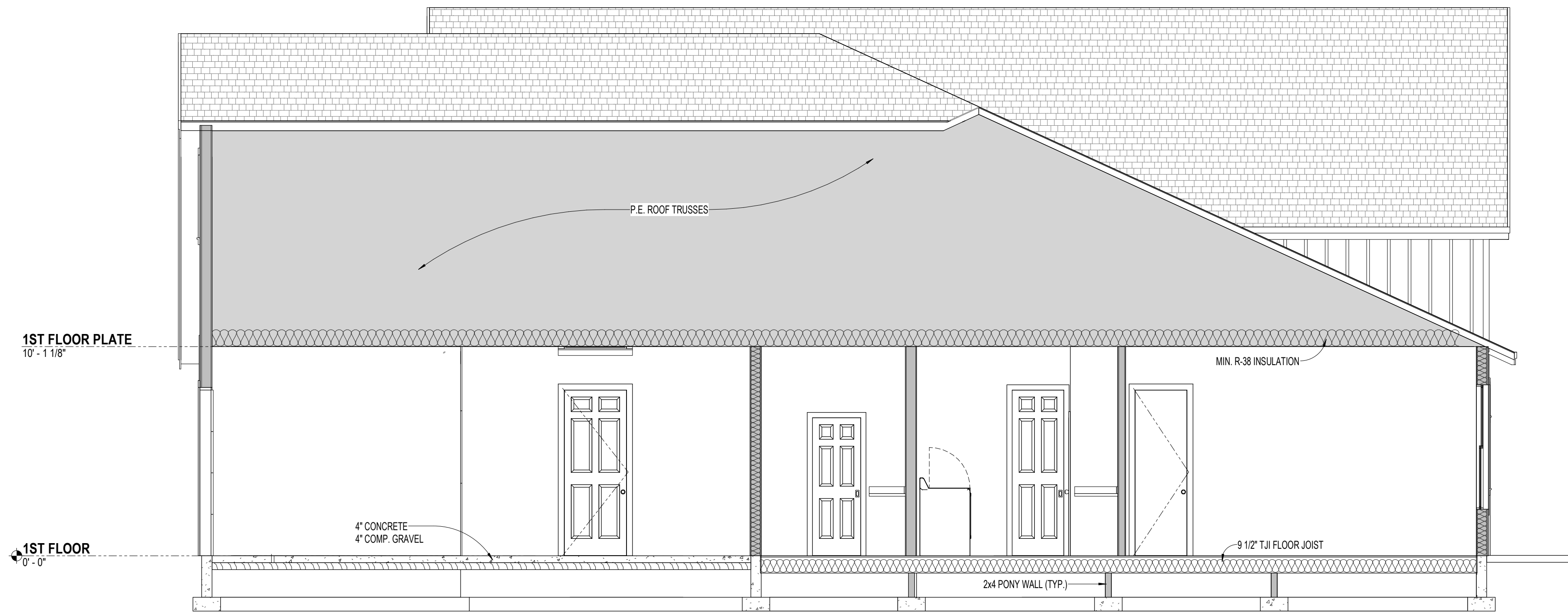
1 BUILDING SECTION-1 1/4" = 1'-0"
