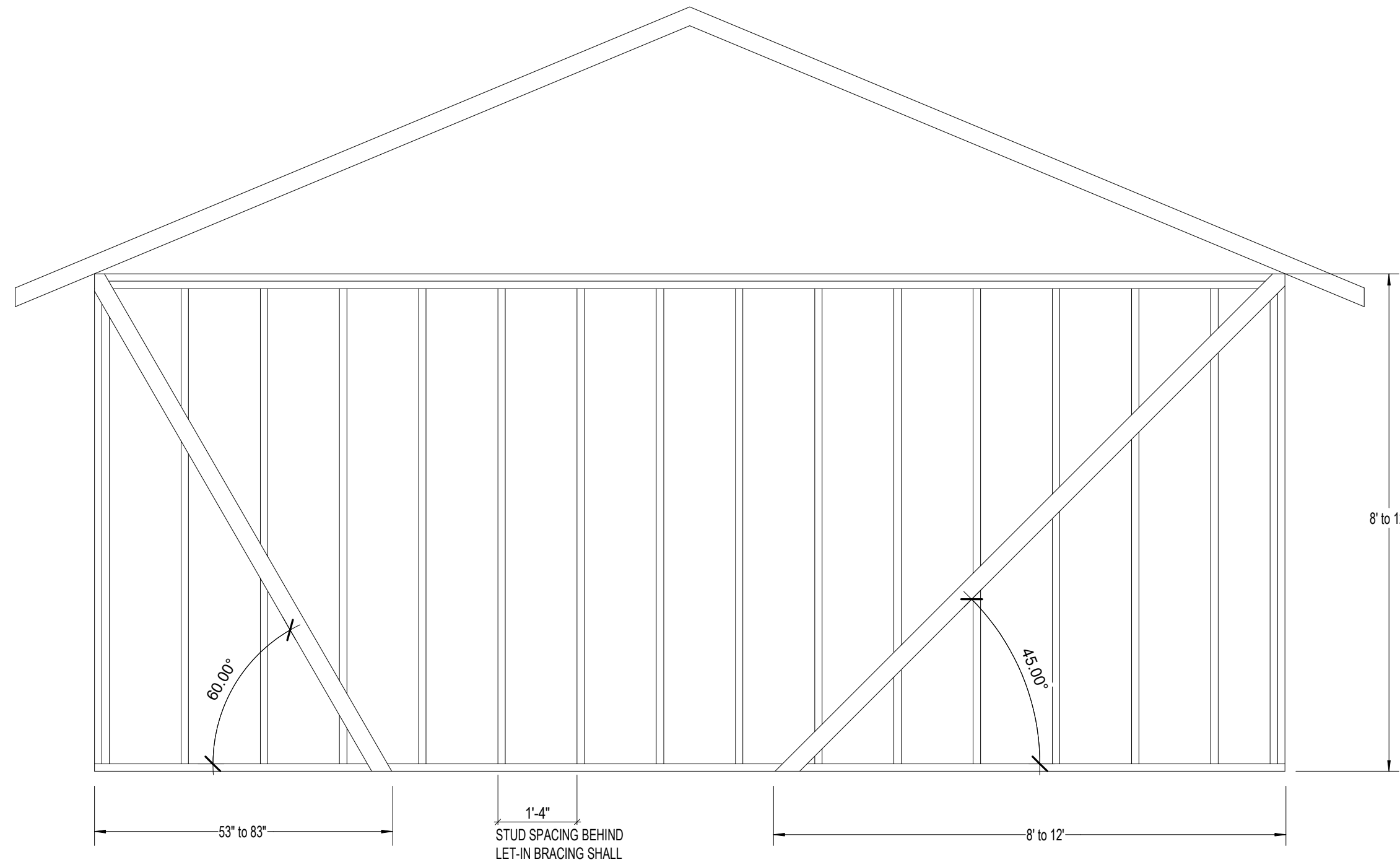
3 LIB DETAIL 1/2" = 1'-0"
