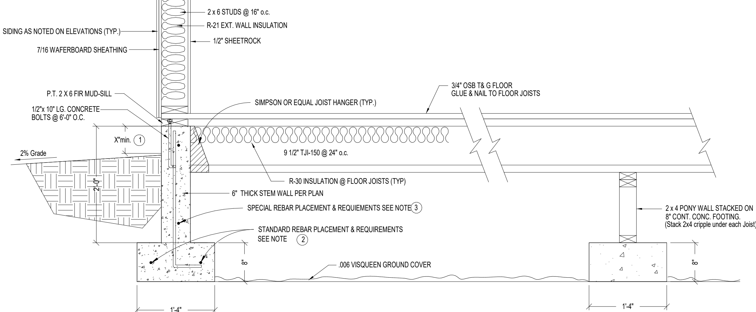
1 WALL SECTION 1" = 1'-0"
