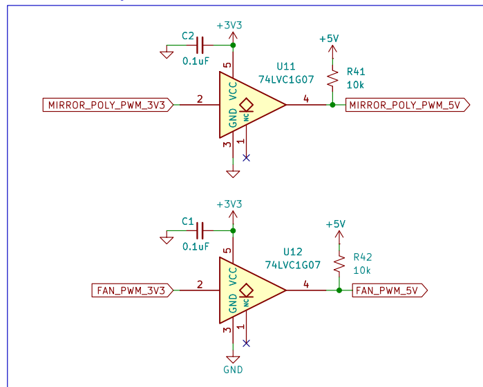
PWM 3V3->5V Logic
