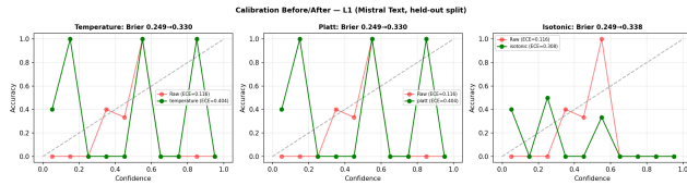
Figure 7: Calibration reliability diagrams (temperature/Platt/isotonic scaling vs. raw) for the L1 (Mistral text) DAIC classifier, held-out split. Monotonic recalibration changes reliability but not ranking-based discrimination.
