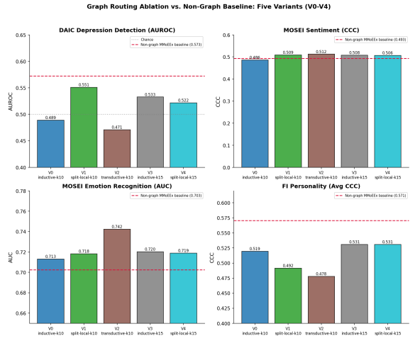
Figure 4: Graph routing ablation vs. non-graph MMoEE baseline (red dashed line), all five variants across all four tasks.
