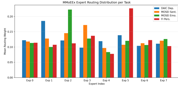
Figure 7: Mean MMoEE routing weight per expert and task (non-graph baseline). Rows/legend are tasks; columns are the 8 experts.
