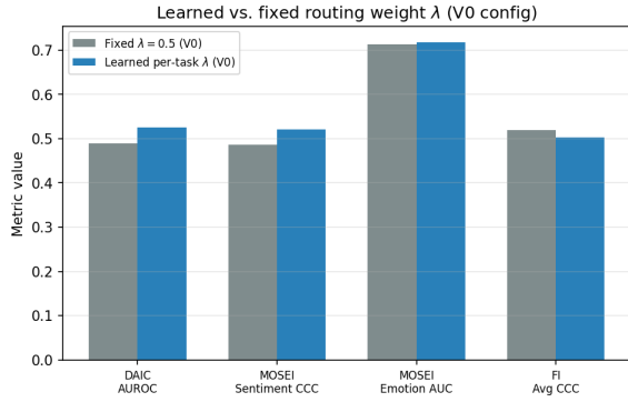
Figure 3: Learned per-task \lambda (V0 configuration, values 0.479–0.574) vs. the fixed default (0.5): a real gain on DAIC (AUROC 0.489 \rightarrow 0.525, still short of the 0.573 non-graph baseline) but not on FI (CCC 0.519 \rightarrow 0.503, moving further from the 0.571 baseline).
